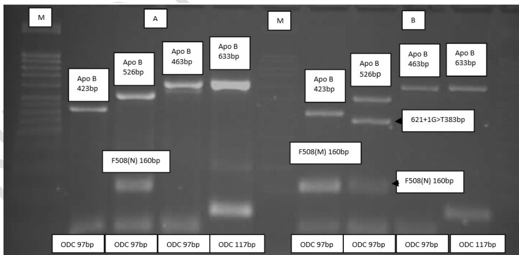
Figure 1. M- molecular weight marker (50 bp ladder); A- patient with normal \Delta F508(N) allele; B- patient with heterozygous for the mutation \Delta F508(M) allele and the 621+1G>T383 mutation; ApoB-Upper control; ODC-lower control
