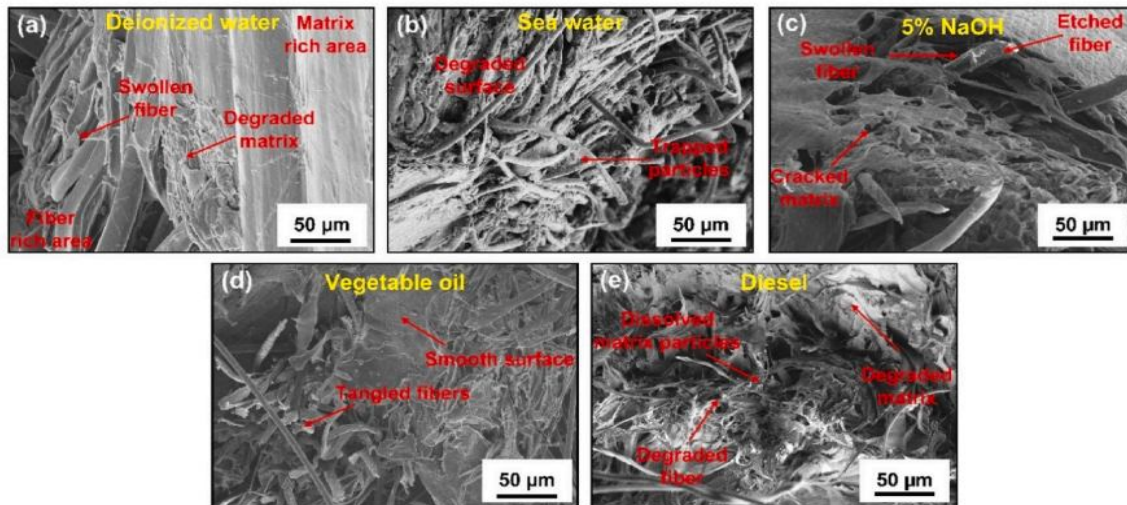
Fig. 8 Examined the long-term stability of kenaf fiber-reinforced polymer composite under various conditions over the course of six months using SEM micrographs[143]
