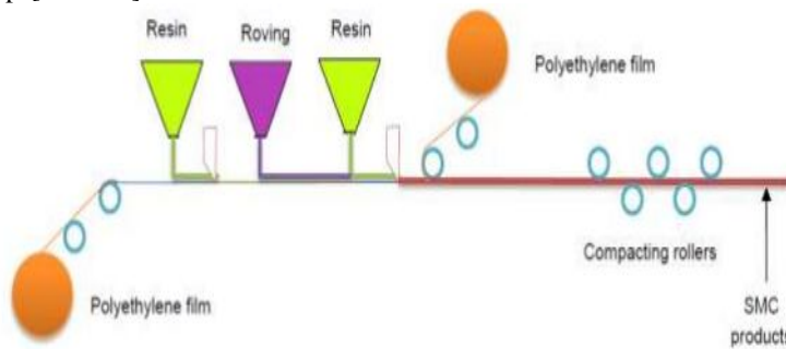
Fig. 7 Manufacturing process of SMC
