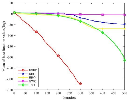
(c) f_3 average convergence curve
