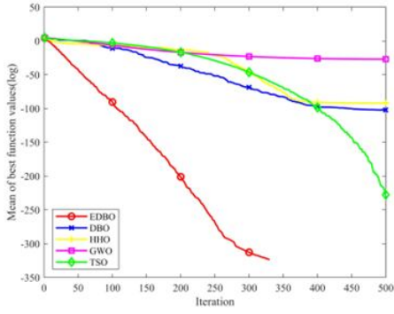
(a) f_1 average convergence curve
