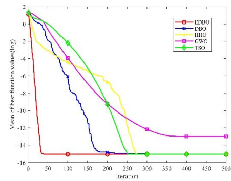
(h) f_8 average convergence curve
