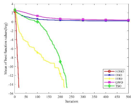
(g) f_7 average convergence curve
