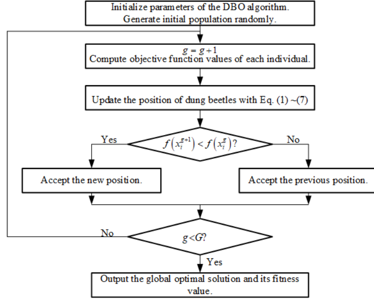
Fig. 1. The flowchart of the DBO algorithm
