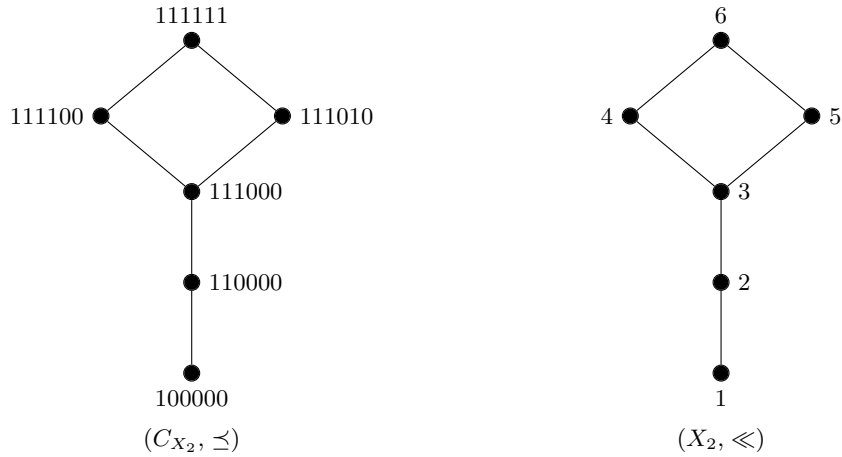
Figure 3.2: Graphs of (C_{X_2}, \preceq) and (X_2, \ll) .
