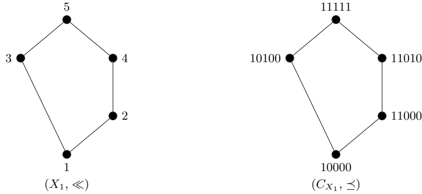
Figure 3.1: Graphs of (X_1, \ll) and (C_{X_1}, \preceq) .
