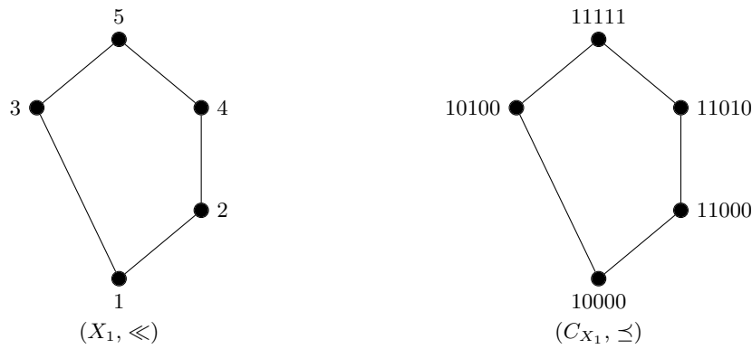
Figure 1: Graphs of (X_1, \ll) and (C_{X_1}, \preceq) .
