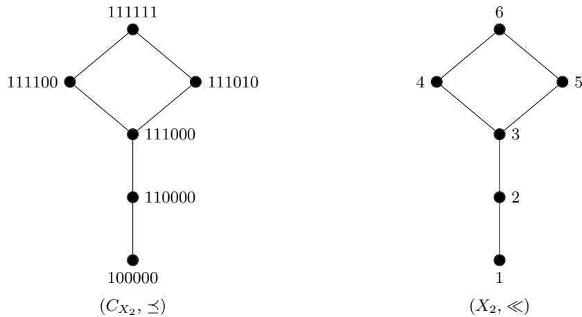
Figure 2: Graphs of (C_{X_2}, \preceq) and (X_2, \ll) .
