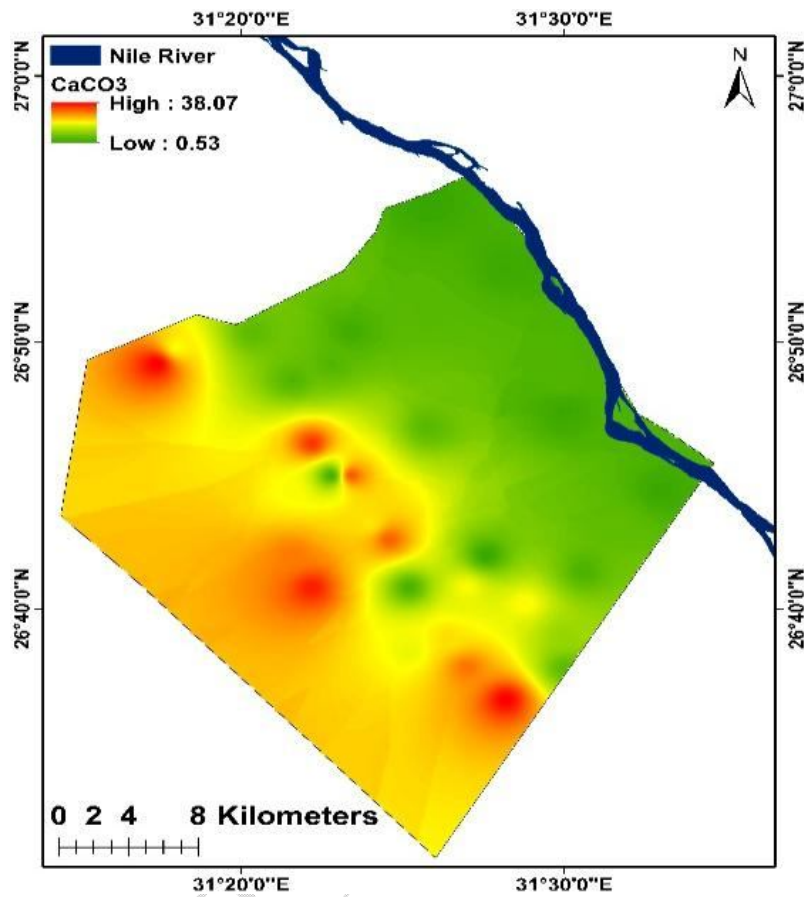
Figure 12. The spatial distribution maps \text{CaCO}_3
