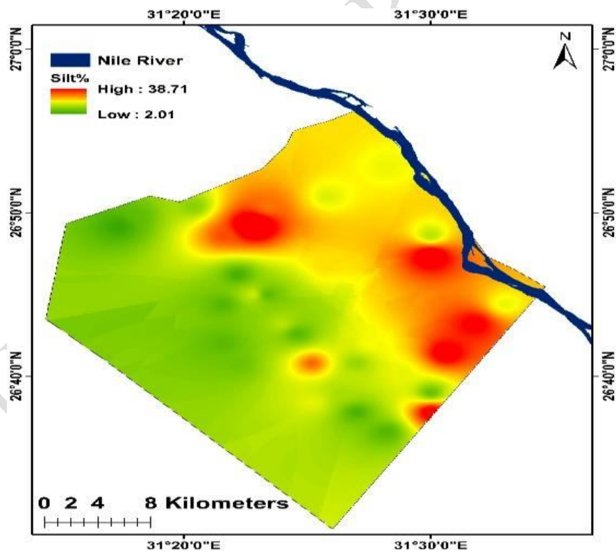
Figure 5. The spatial distribution maps of silt
