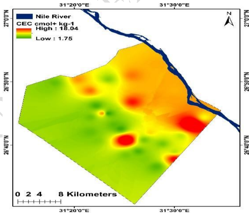
Figure 7. The spatial distribution maps of CEC
