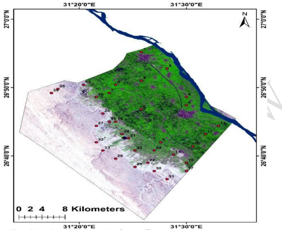
Figure 2. Location of the soil samples.
