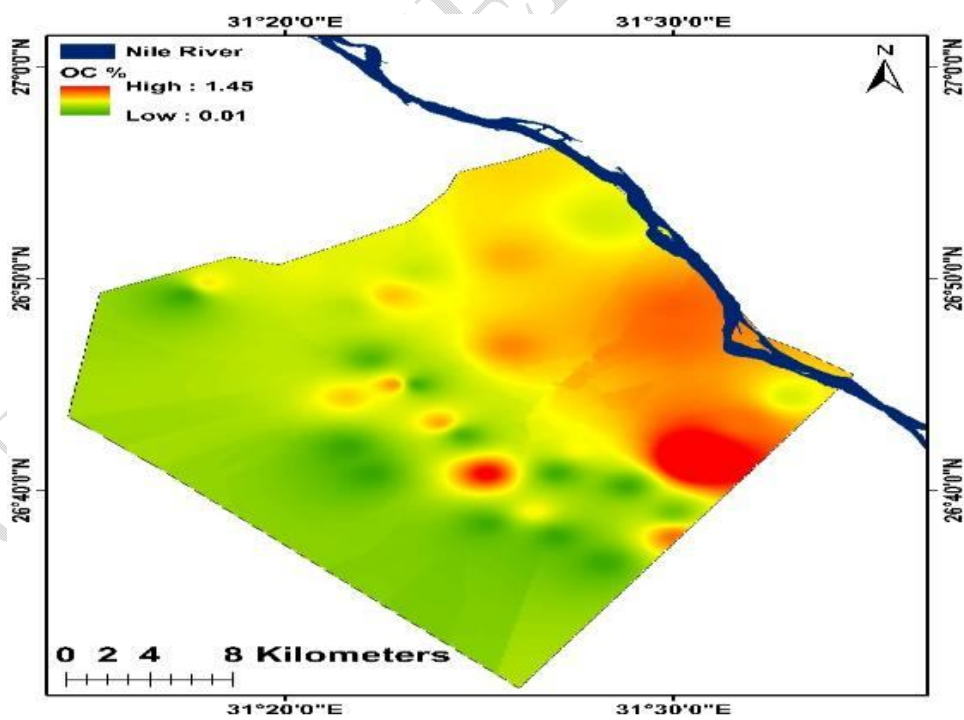
Figure 9. The spatial distribution maps of OC
