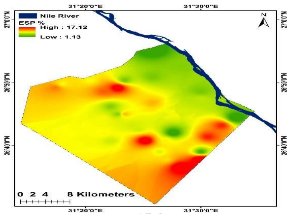
Figure 8. The spatial distribution maps of ESP
