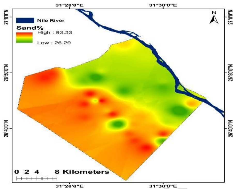
Figure 4. The spatial distribution maps of sand
