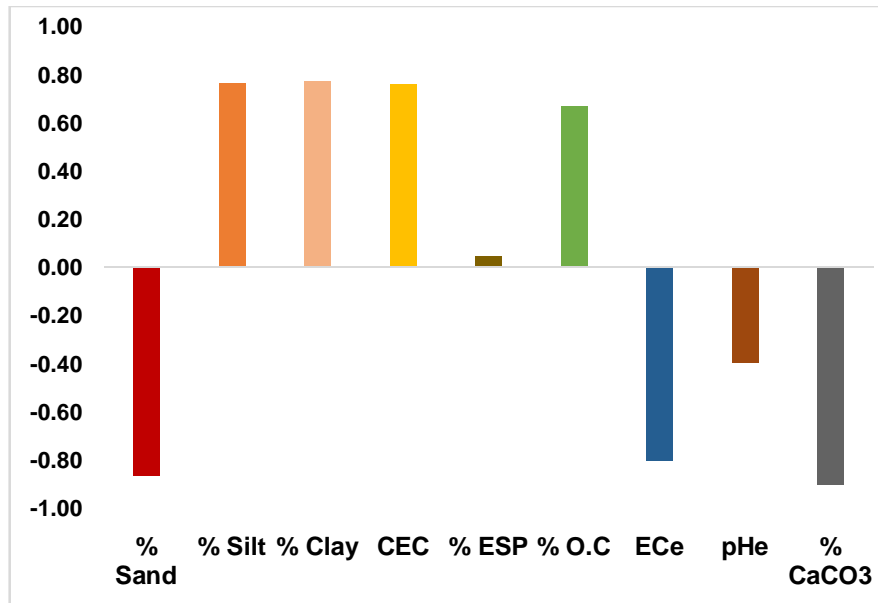
Figure 14. Correlation coefficients between the different soil indicators and SQI
