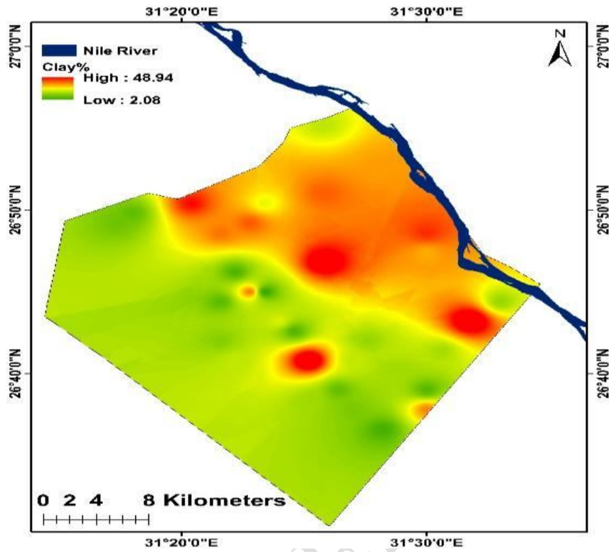
Figure 6. The spatial distribution maps of clay
