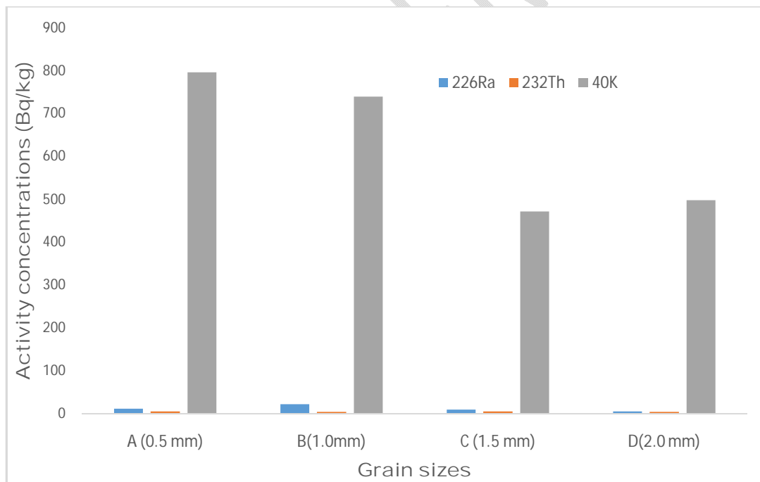
Fig 4: Variations of activity concentration of ^{226}\text{Ra} , ^{40}\text{K} and ^{232}\text{Th} with grain sizes from Kolo samples
