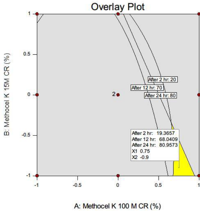
Figure 5 The overlay plot of the optimization area.
