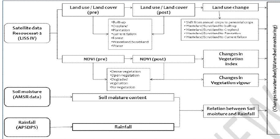
Fig. 2. Methodology workflow
