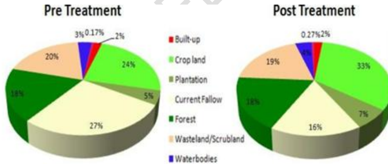
Fig 5: Land use land cover maps comparison
