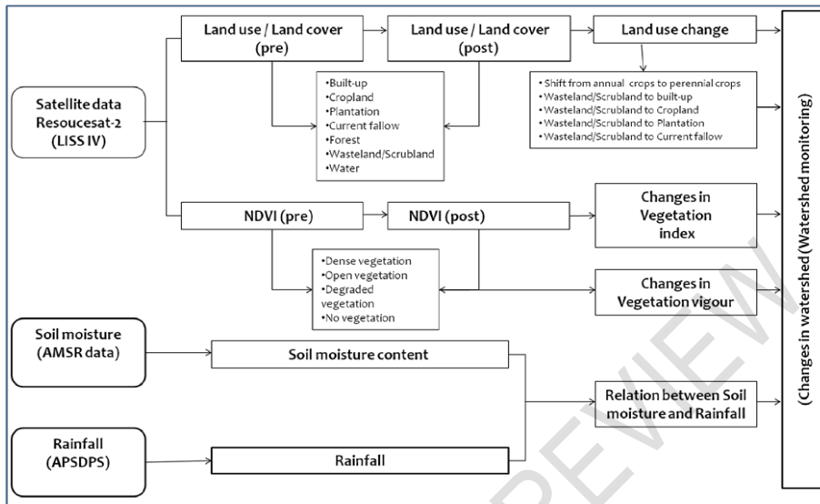
Fig 1: Methodology adopted for the study
