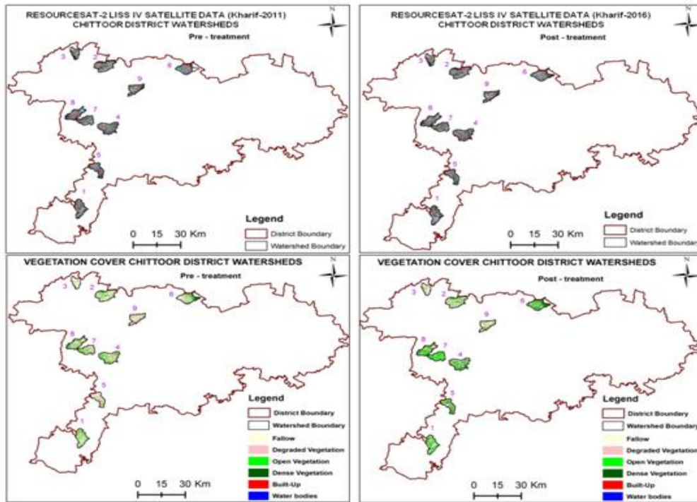
Fig 2: Comparison of Vegetation Cover maps
