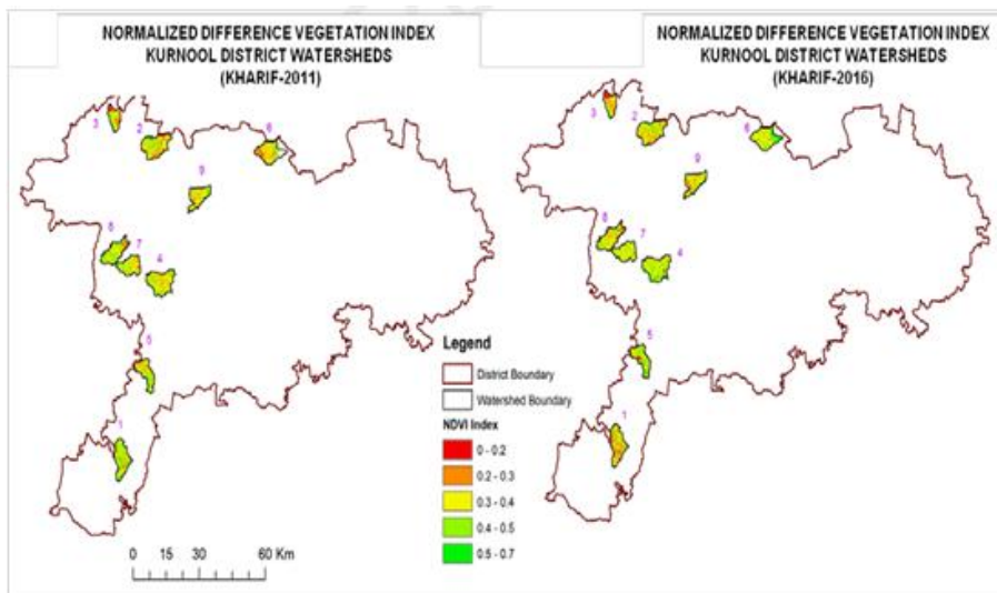
Fig 4: Normalized difference vegetative index comparison for 2011 and 2016
