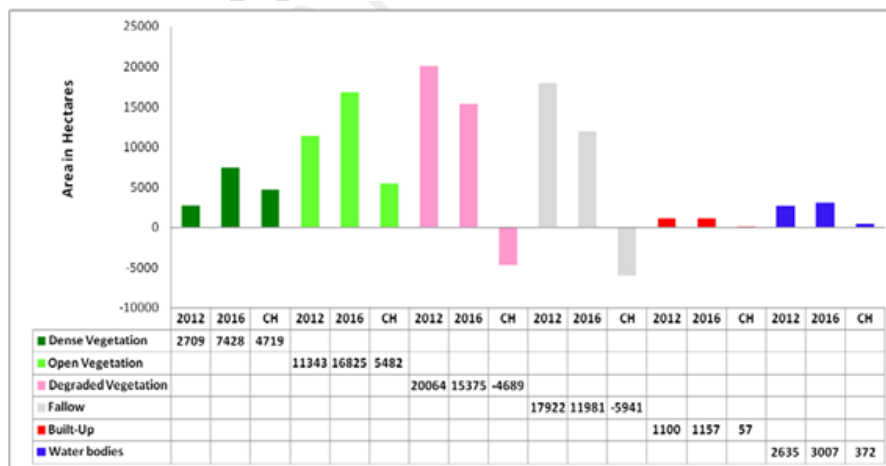
Fig 2: Comparison of Vegetation Cover maps
