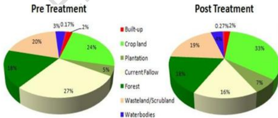
Fig 5: Land use land cover maps comparison
