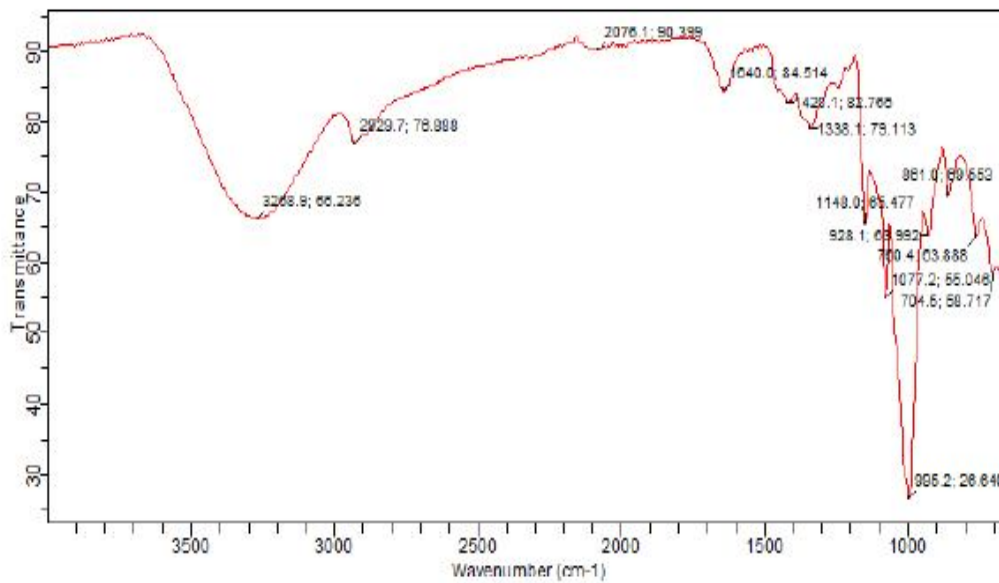
Figure 1b. FARO 40 Phosphorylated Starch Fourier Transform Infrared Spectroscopy Spectral
