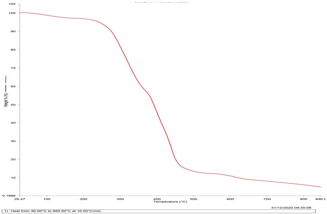
Figure 2b. FARO 40 Phosphorylated Starch Thermogravimetric Analysis Plot
