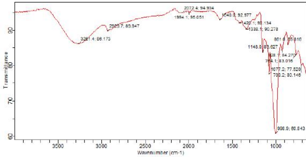
Figure 1a. FARO 40 Native Starch Fourier Transform Infrared Spectroscopy
