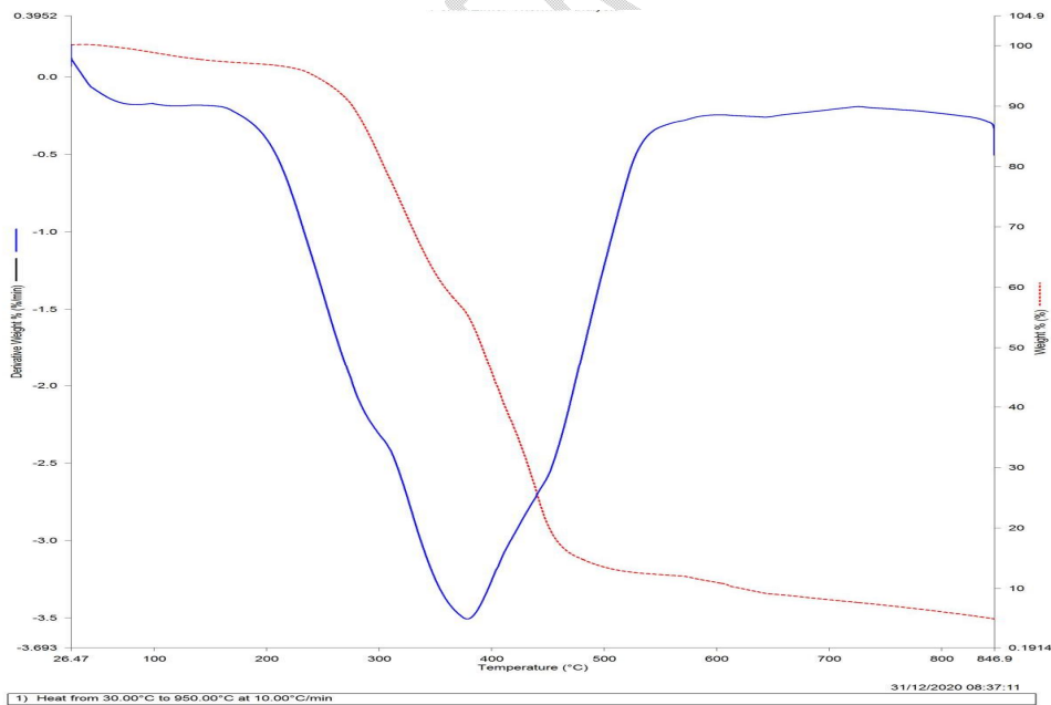
Figure 3b. FARO 40Phosphorylated StarchDerivative Thermogravimetric Plot
