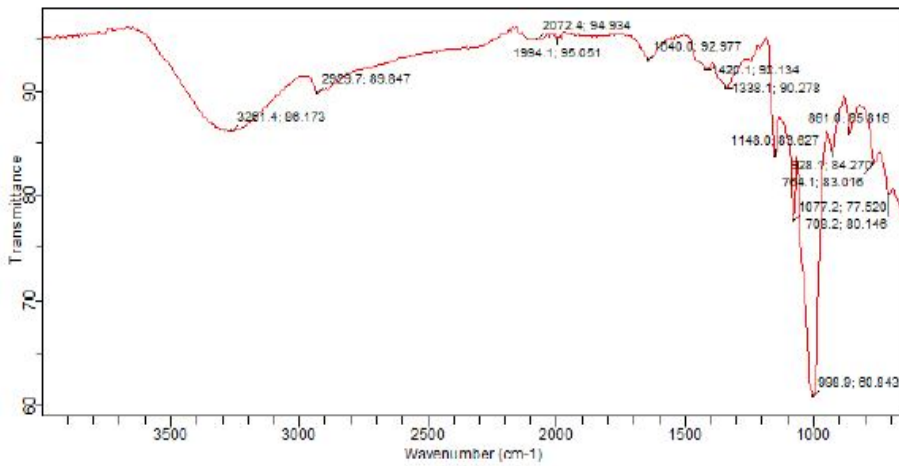
Figure 1a. FARO 40 Native Starch Fourier Transform Infrared Spectroscopy Spectral
