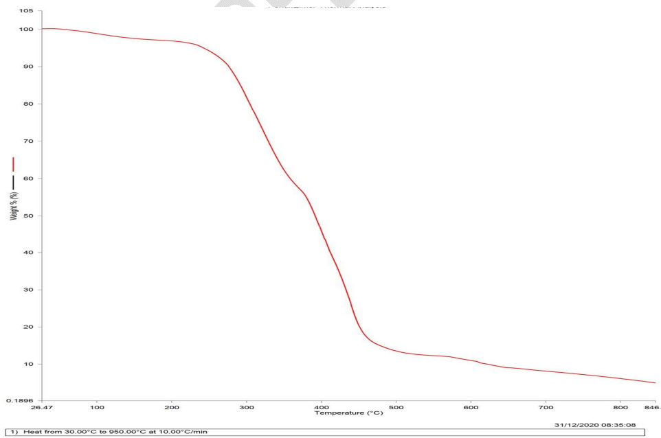
Figure 2b. FARO 40 Phosphorylated Starch Thermogravimetric Analysis Plot
