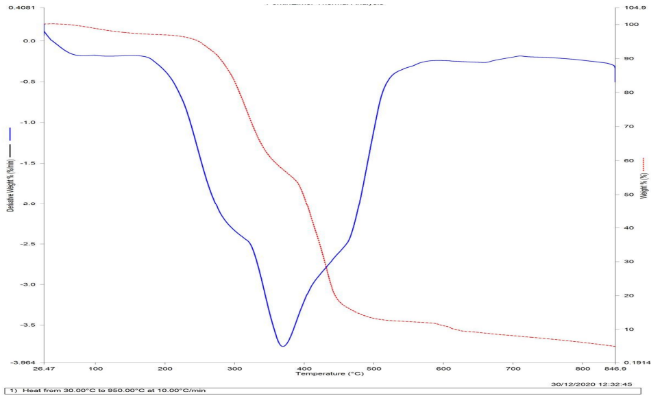
Figure 3a FARO 40 Native StarchDerivative Thermogravimetric Plot
