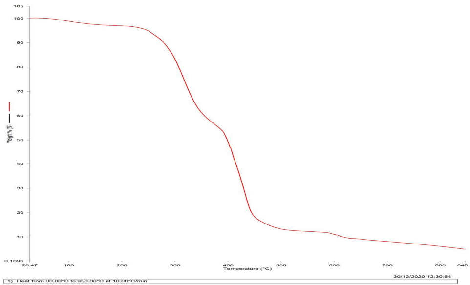
Figure 2a. FARO 40 Native Starch Thermogravimetric Analysis Plot
