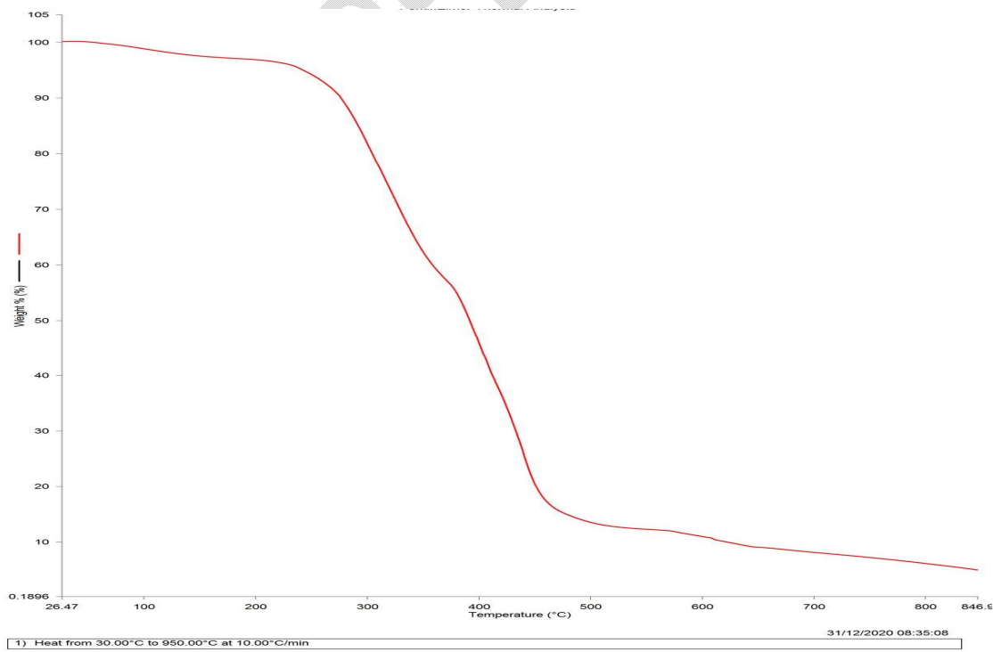
Figure 2b. FARO 40 Phosphorylated Starch Thermogravimetric Analysis Plot
