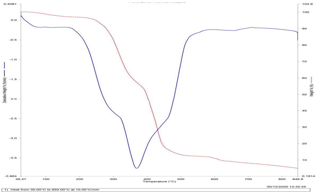
Figure 3a FARO 40 Native Starch Derivative Thermogravimetric Plot
