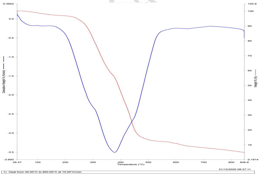
Figure 3b. FARO 40 Phosphorylated Starch Derivative Thermogravimetric Plot
