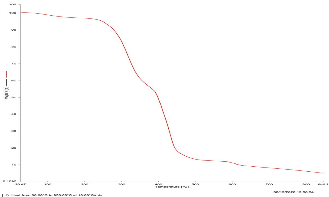
Figure 2a. FARO 40 Native Starch Thermogravimetric Analysis Plot
