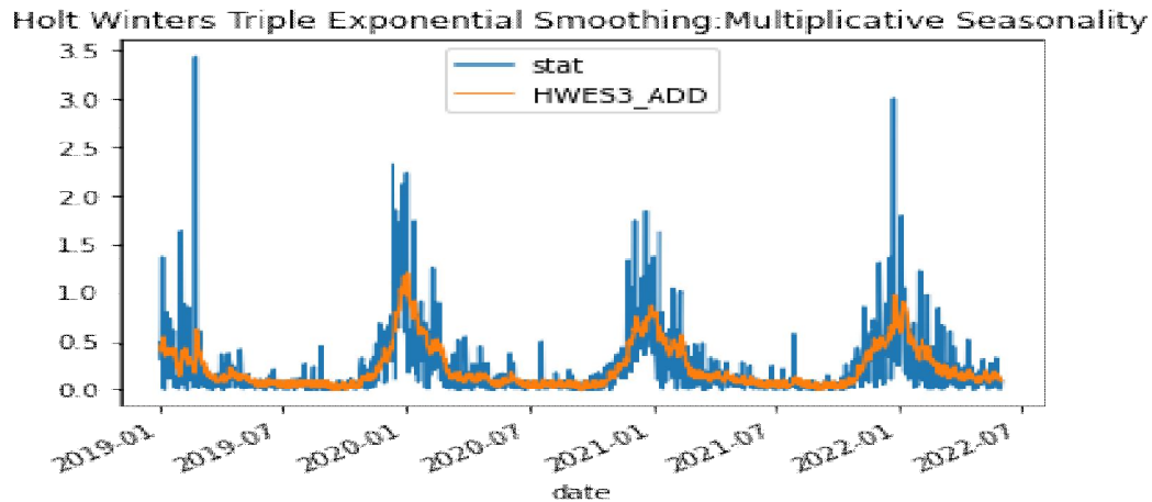
Fig. 3 Holt Winter's model on Sulphur Dioxide
