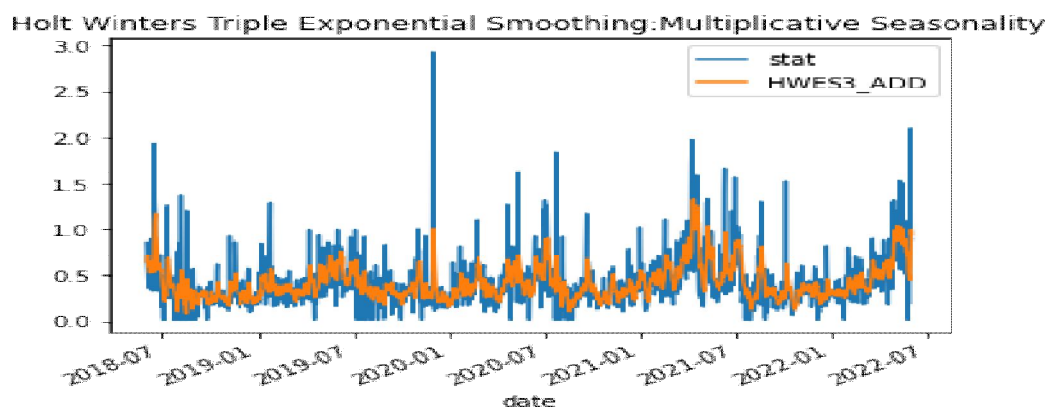
Figure 12. Holt Winter's model on AOD
