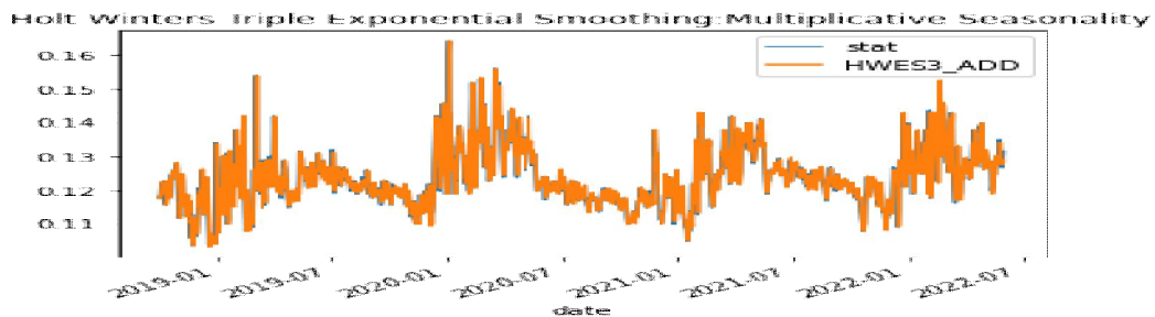
Fig. 2 Holt Winter's model on Ozone
