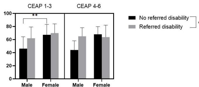
Fig.1.- Three-way analysis of variance, vertical axis being age.
