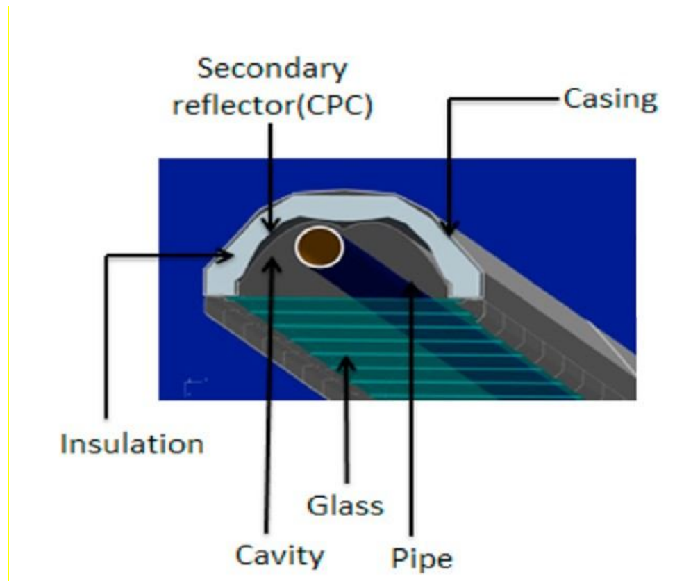
Figure 2. Receiver for LFC with secondary concentrator [11]
