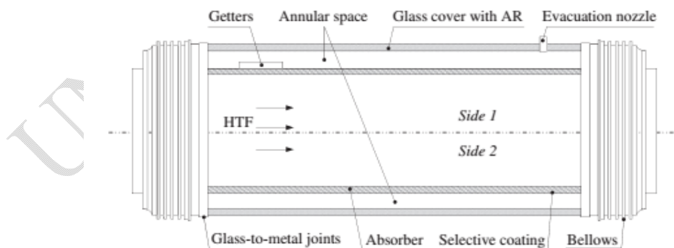
Figure 3: vacuum absorber tube [38].
