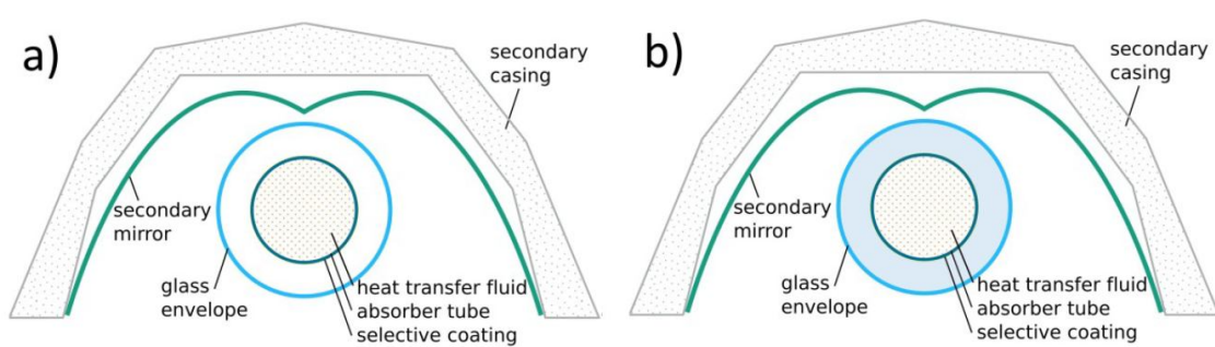
Figure 12: Mono-tube receiver with CPC secondary concentrator a) non- vacuum absorber, b) vacuum absorber [49].
