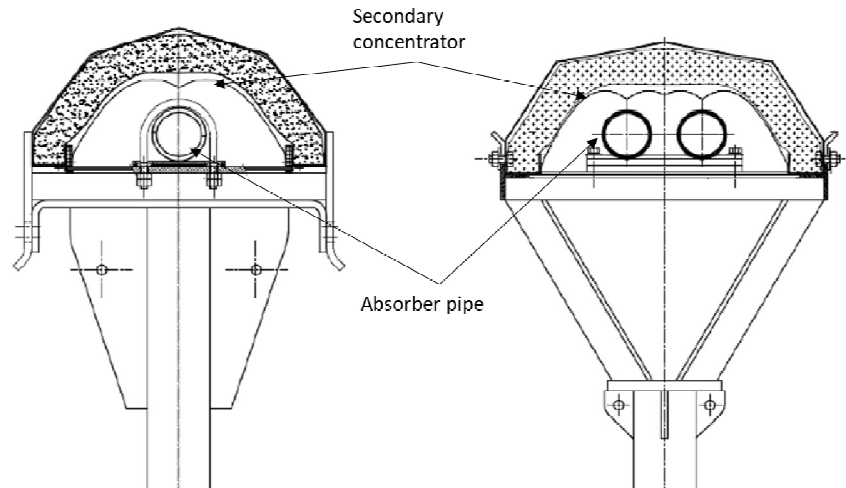
Figure 156. using of two absorbers two instead of one with a CPC secondary concentrator [11].
