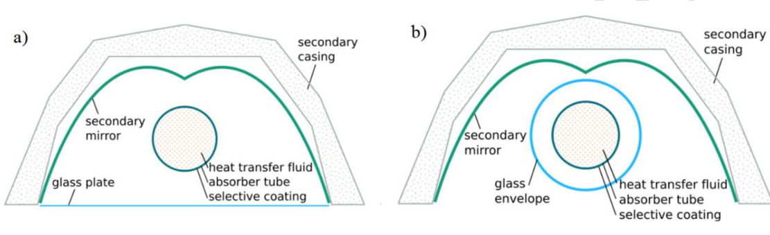
Figure 13: Receiver with CPC secondary concentrator a) glass plate cover; b) glass envelope cover [50].
