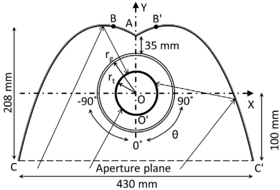
Figure 14. Receiver with CPC secondary concentrator allowing to irradiate the upper of absorber [42]
