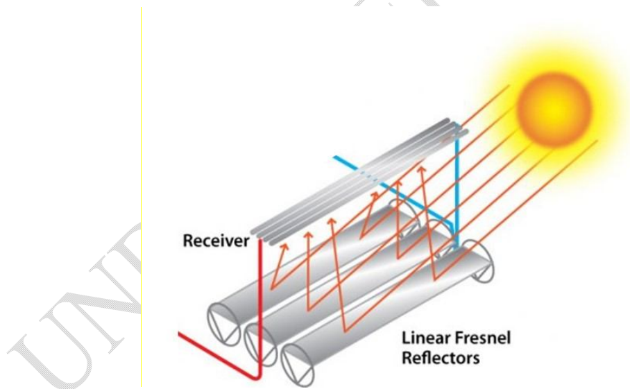
Figure 1: A LFR overview [6].
