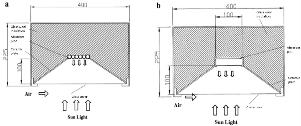
Figure 224: Two identical receivers one with multi-tube absorber the other with plan absorber [14].
