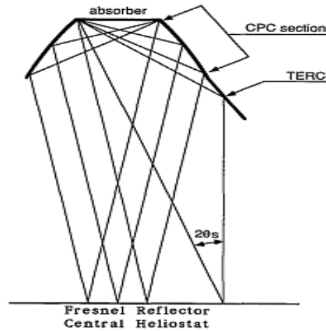
Figure 9. Gordon et al. trapezoidal secondary concentrator [27].
