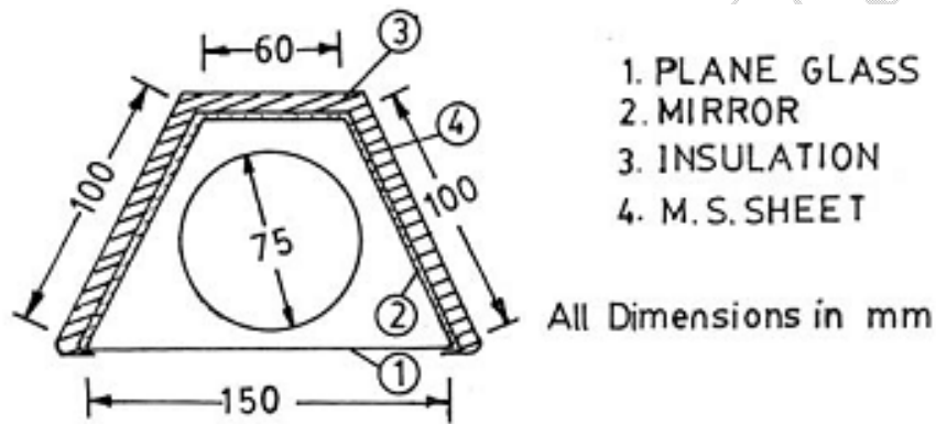
Figure 10: Non-vacuum mono-tube absorber with trapezoidal secondary concentrator and glass cover [45].
