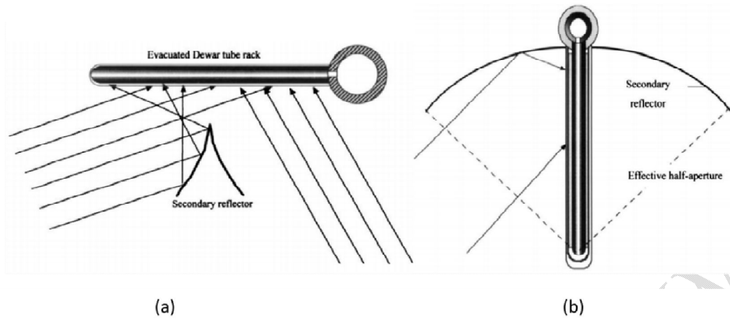
Figure 191: Dewar tubes receiver: a) horizontal orientation; b) vertical orientation [7].
