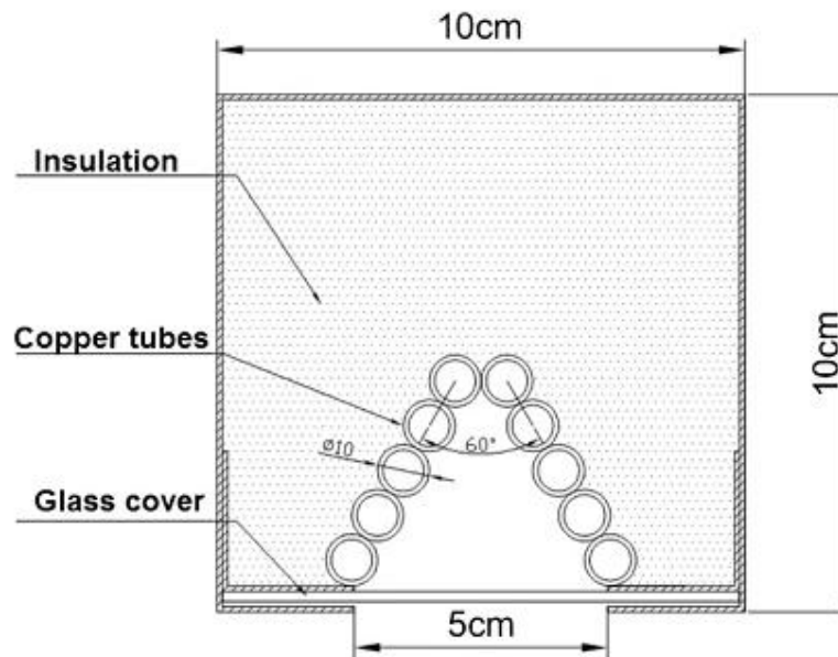
Figure 180: Reverse V-shape or triangular receiver [60].
