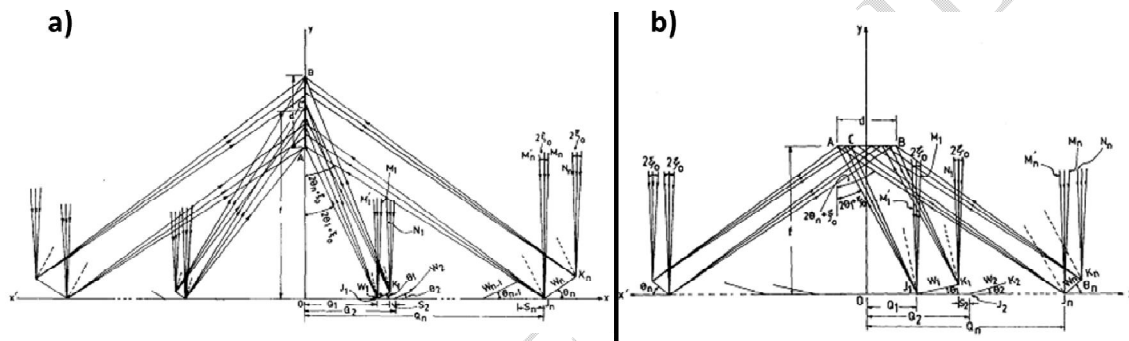
Figure 202: plan absorber a) vertical [30] and b) horizontal [29].
