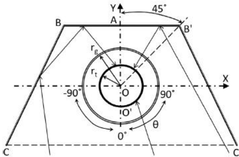
Figure 8. Mono-tube absorber with trapezoidal secondary concentrator used to refocus on absorber sun ray that missed the absorber after a first reflection on principal concentrator [42]
