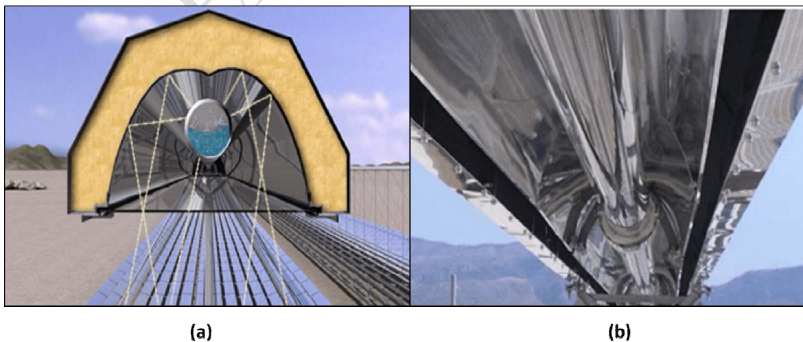
Figure 11. Mono-tube receiver of Novatec Solar with CPC secondary concentrator a) Nova-1 non- vacuum absorber used for Puerto Errado 2 power plant [46], b) Supernova with vacuum absorber
