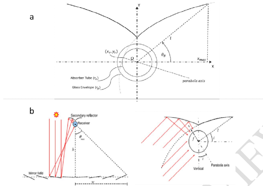
Figure 6: vacuum tubular absorber with butterfly secondary concentrator: a)[41] b) [33].
