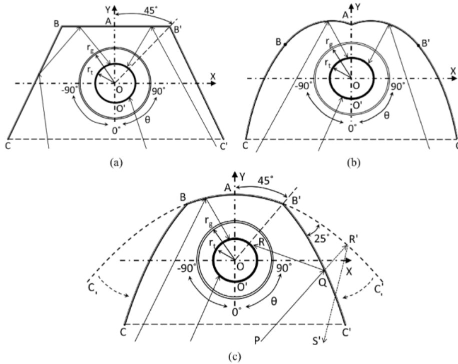
Figure 15. Different profiles of secondary concentrator (a) Trapezoidal Concentrator (b) Compound parabolic concentrator and (c) Segmented Parabolic secondary Concentrator [42]
