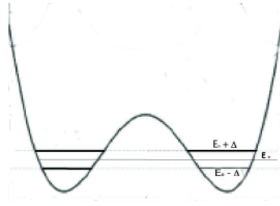
PIc 3: The schematic representation of the potential well with two symmetric states. In the ground state, electron can be either in the right or in the left hole. In the unperturbed state, its wave functions are either \varphi_1 or \varphi_2 with the energy E_0 . The quantum tunneling transition from one state to another leads to the splitting of energy level and to the lowering of the sublevel on \Delta .
