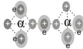
Рис. 8: Schematic representation of energy bonds in the Be-9 core. Dotted lines represent the possibility of a relativistic electron jumping between protons.
