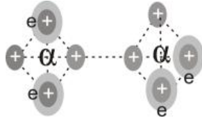
Рис. 7: The schematic representation of energy bonds in the Be-8 core. Dotted lines represent the possibility of a relativistic electron jumping between protons.
