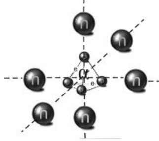
Рис. 11: "Elementary cell" three-dimensional "crystal" models of a heavy nucleus in which alpha particles are "glued" together by neutrons.
