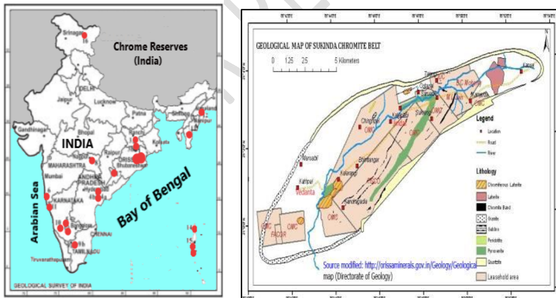
Fig 5: Chrome reserves in India and Chromite mines with leaseholders in SUC, Jajpur district (Source modified: Geological Survey and Directorate of Geology)
