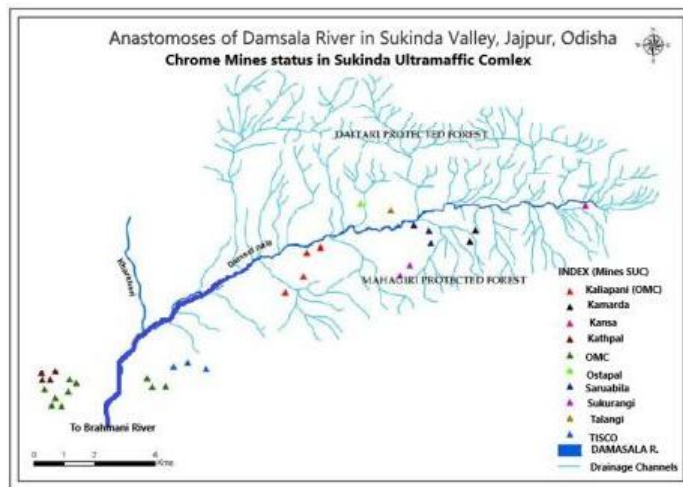
Fig 6: The drainage system of Damsala R. with the chromite mines in SUC. (source modified: EPG: Orissa)
