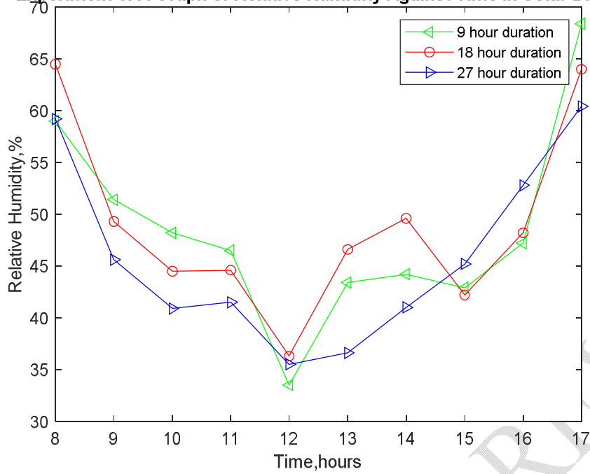
Figure 8: Relative Humidity Against Time Graph in Solar Dryer During Experiment 1
