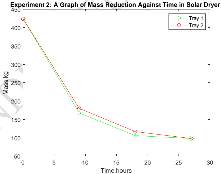
Figure 13: Mass Reduction Against Time Graph in the Solar Dryer During Experiment 2
