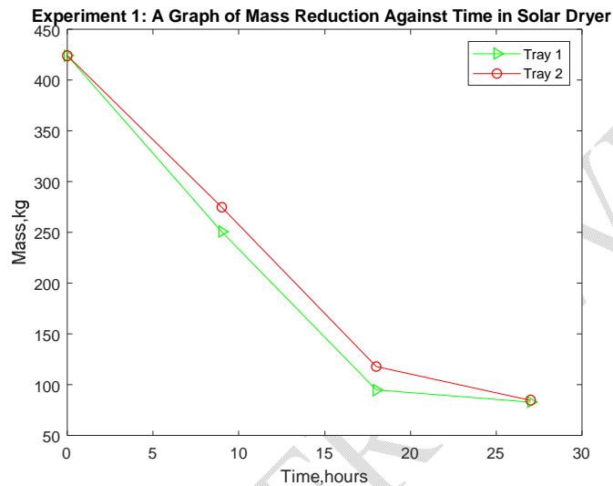
Figure 11: Mass Reduction Against Time Graph in Solar Dryer During Experiment 1
