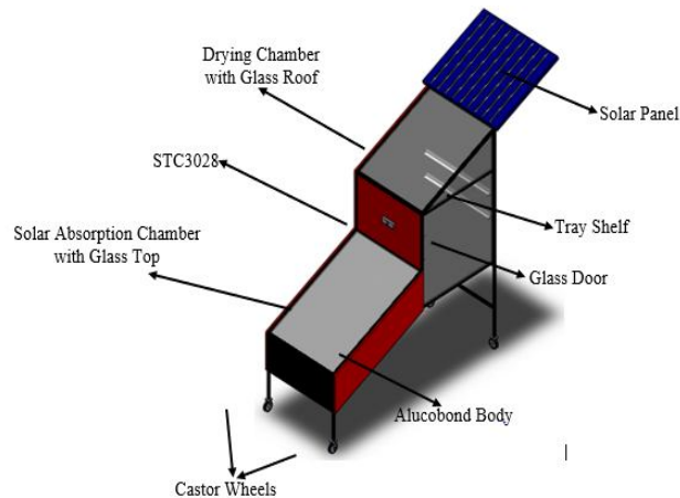
Figure5: SOLID WORK Models of the solar dryer
