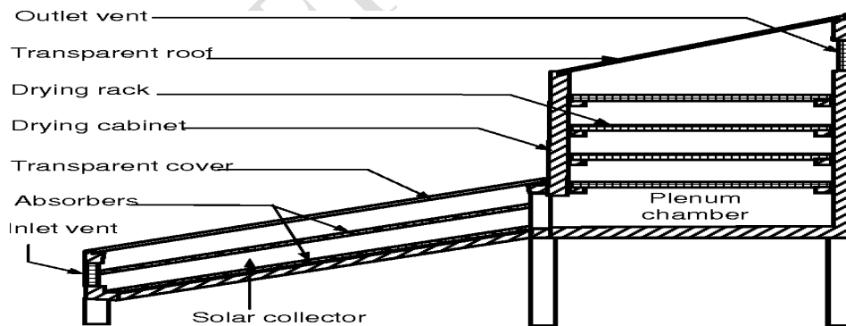
Figure 3: Structure of a Mixed Mode Solar Dryer
