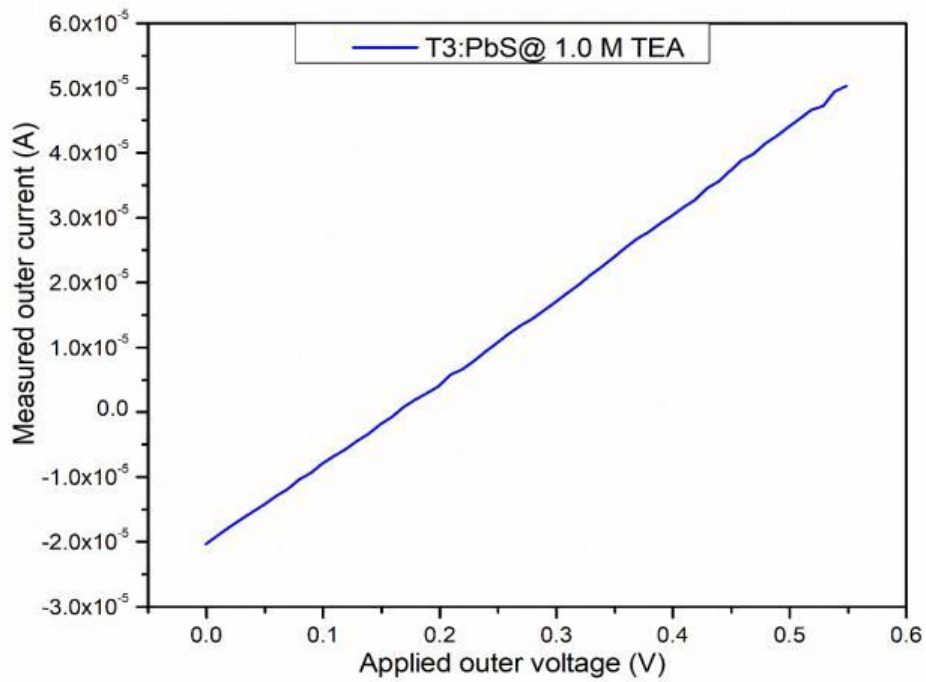
Fig.15: I-V characteristics for T 3 .
