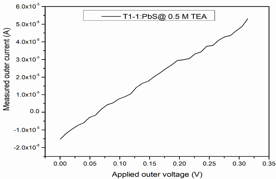
Fig13: I-V characteristics for T 1
