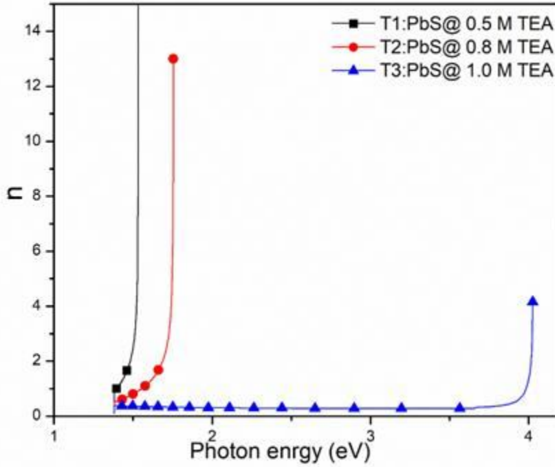
Fig.8: The plot of the Refractive index (n) against the photon energy for sample T 1 , T 2 and T 3 .
