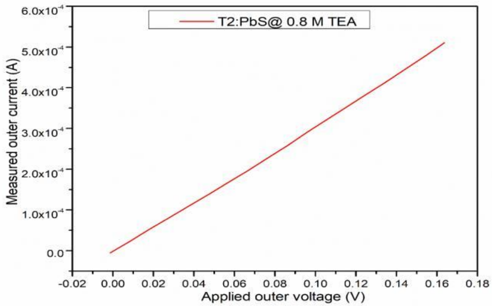
Fig.14: I-V characteristics for T 2 .
