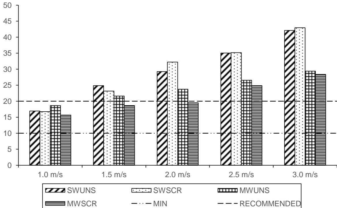
Fig. 2. Ventilation rates ( m^3/h ) in a 100 mm PVC vent pipe fitted to different designs of VIP latrines at varying wind speed thresholds
