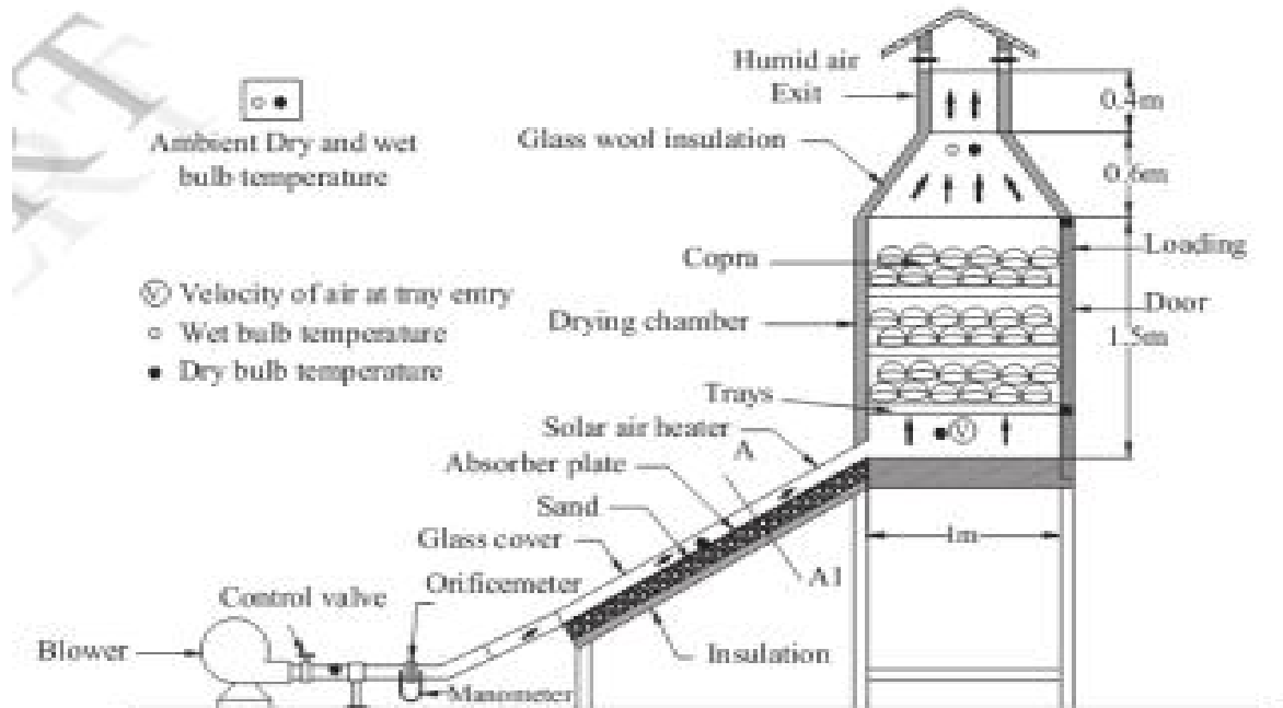
Figure 3. Sectional view of solar drying system used for copra drying
