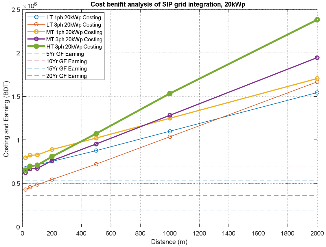
Figure 8: Cost-benefit analysis of a 20kWp SIP grid integration
