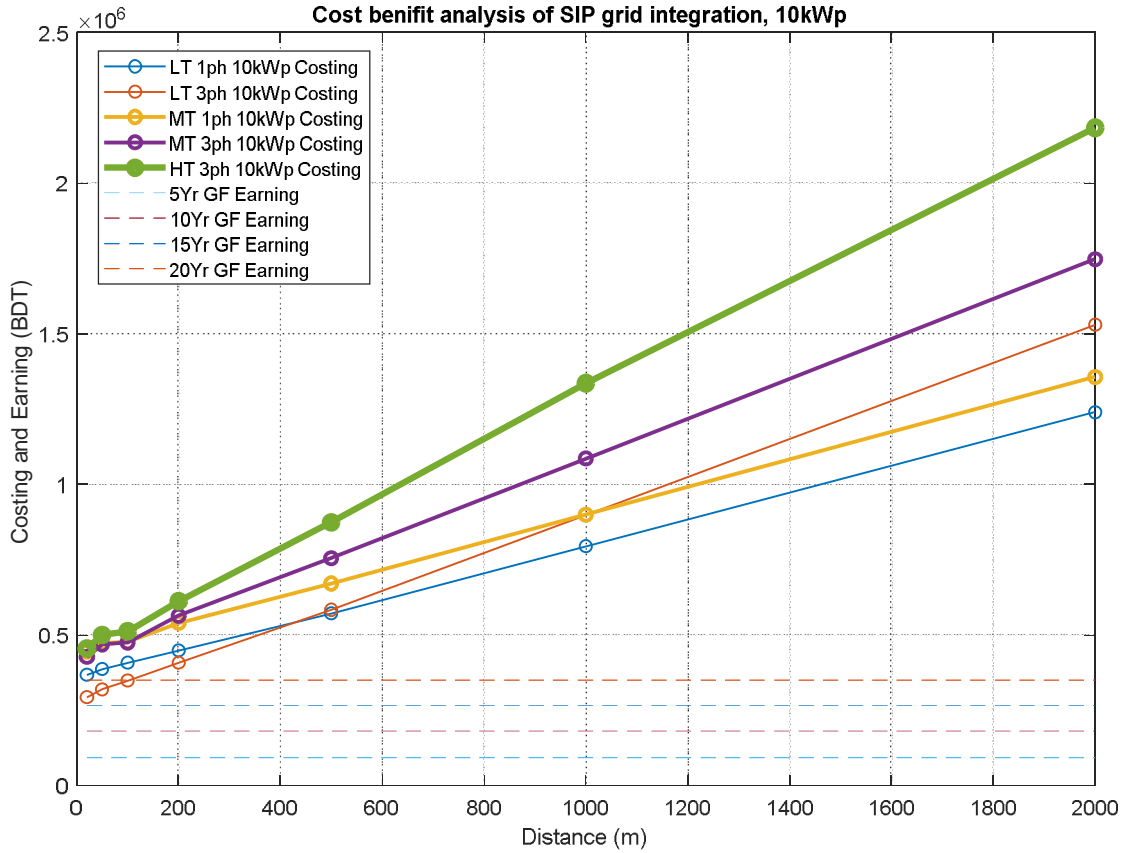
Figure 7: Cost-benefit analysis of a 10kWp SIP grid integration
