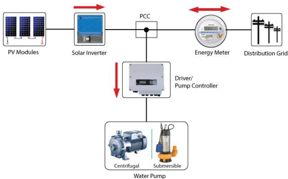
Figure 2: Connection diagram according to the Net Metering Guidelines
