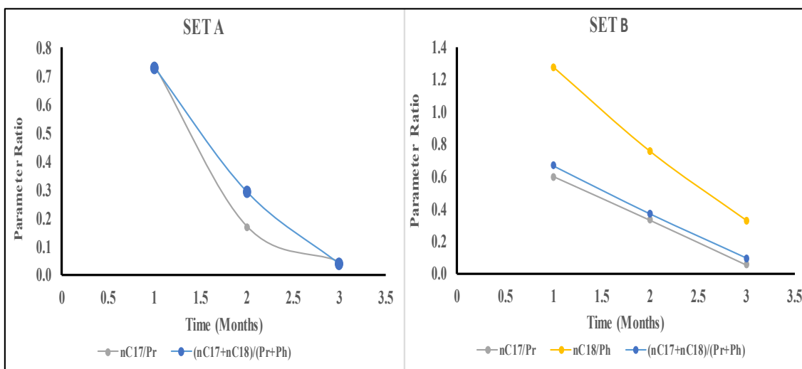
Figure 1. Biostimulated biodegradation profile for sample sets A and B
