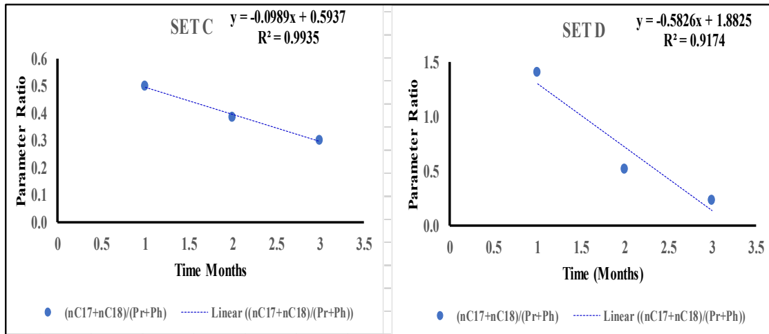
Figure 6. Biostimulated biodegradation models for samples set C and D.
