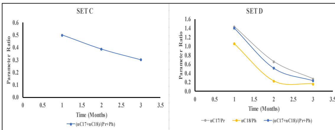
Figure 2. Biostimulated biodegradation profile for sample sets C and D
