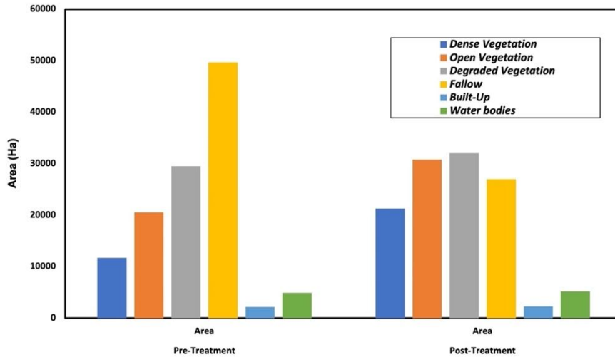
Figure 3a. Changes in Vegetation cover
