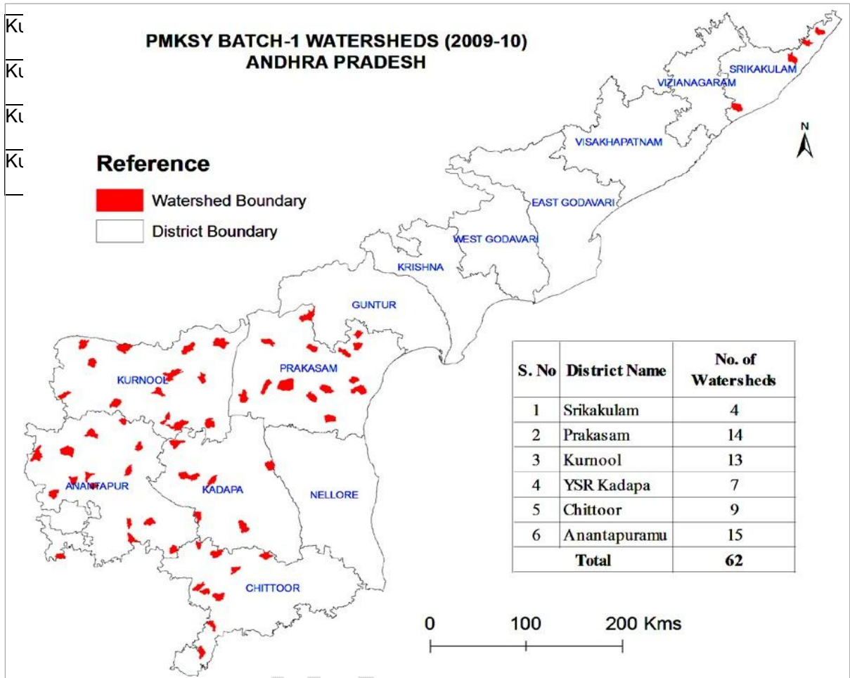
Figure 1. Location map of watersheds
