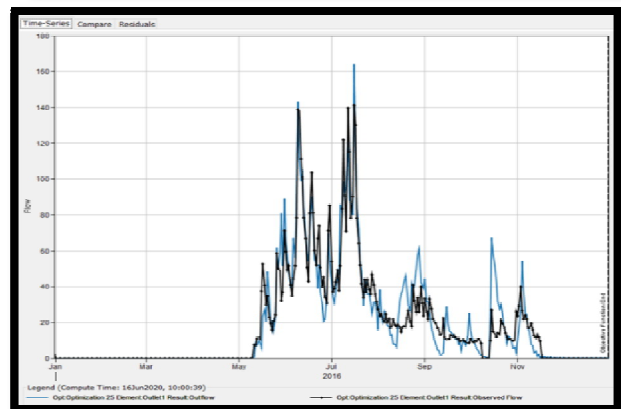
Fig. 6 Simulated and observed hydrograph during calibration period
