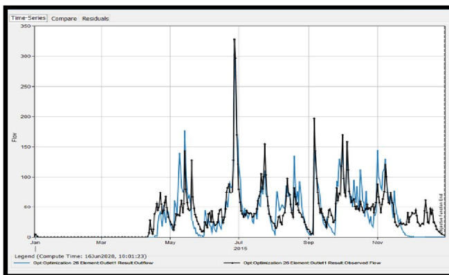
Fig. 6 Simulated and observed hydrograph during calibration period
