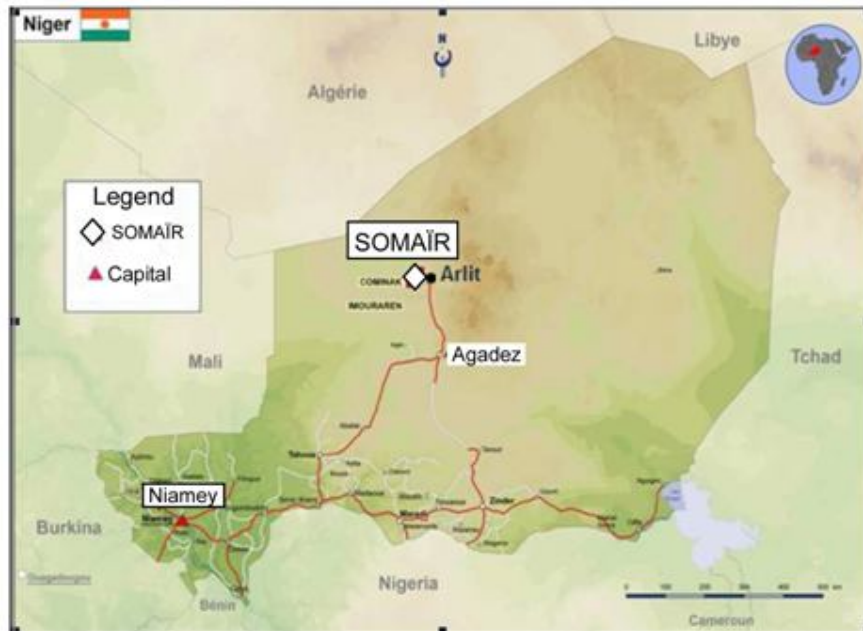
Figure 1: Location of the SOMAÏR mine [15]
