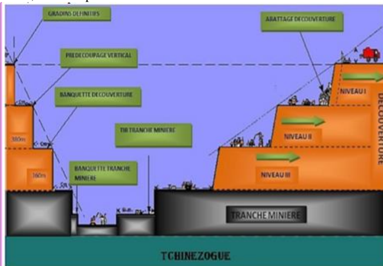
Figure 2: Schematic cross-section of mining at SOMAÏR [16]
