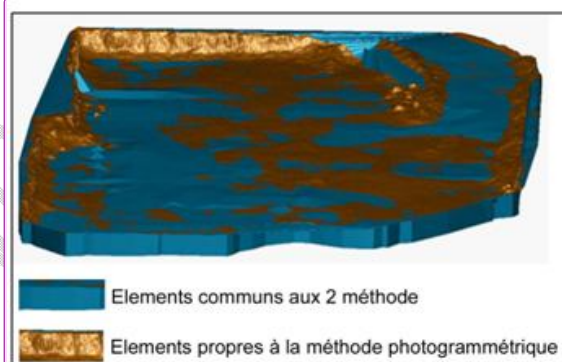
Figure 9: DTM image comparing topographic and photogrammetric methods
