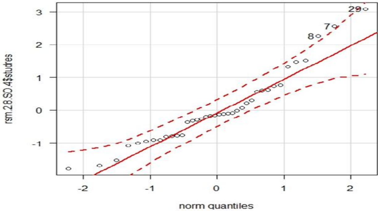
Figure 5: Normality of Residuals
