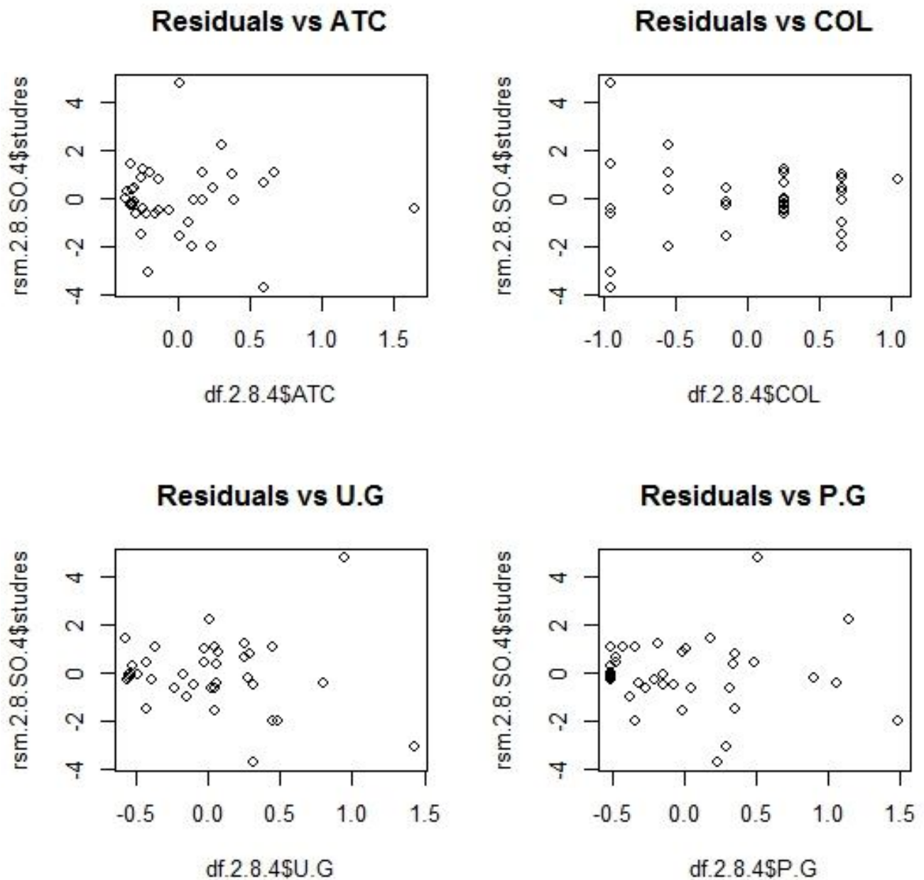
Figure 5. RESIDUALS PLOT OF ATC, COL, U.G, and P.G
