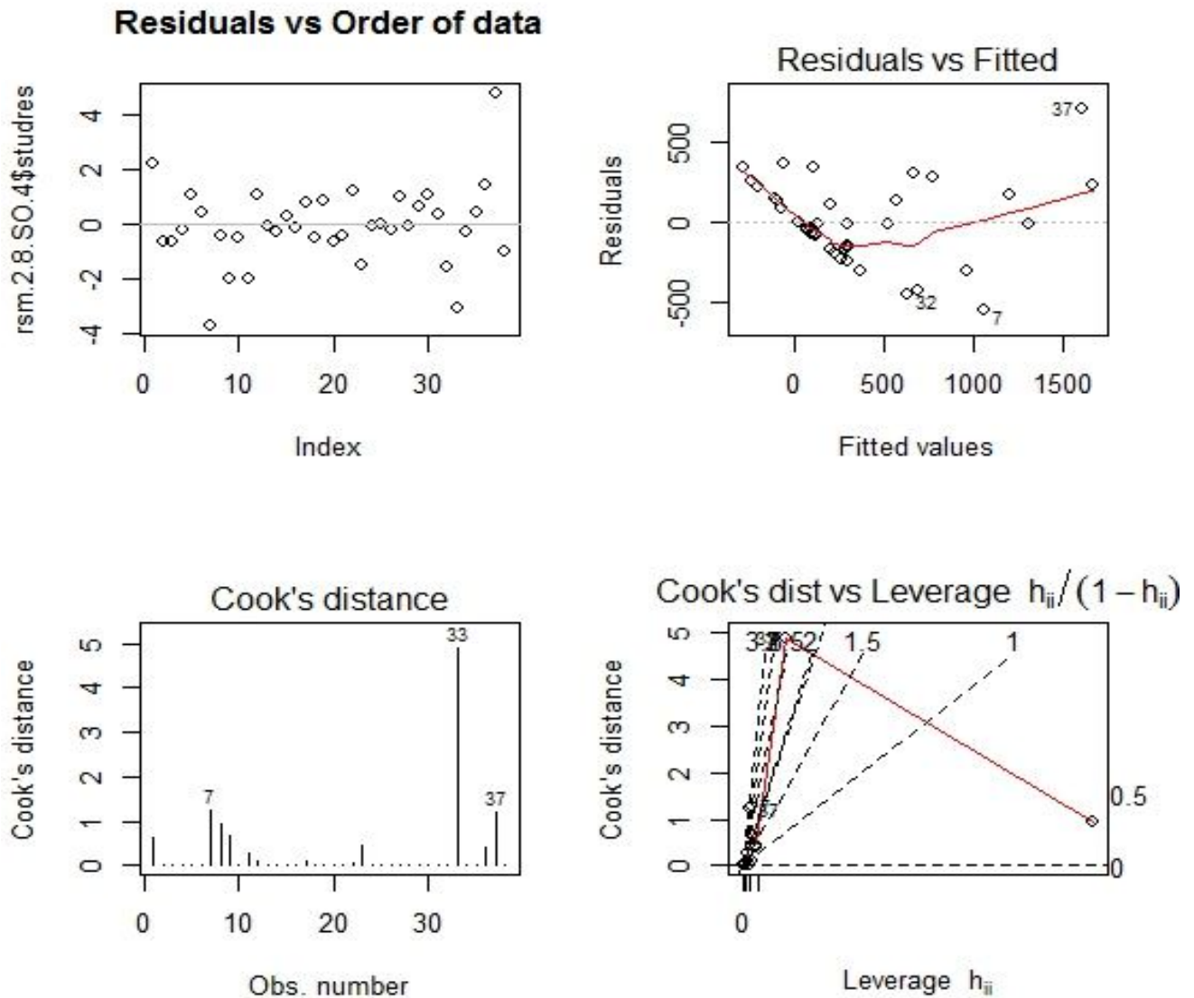
Figure 4: Residuals vs. order of data
