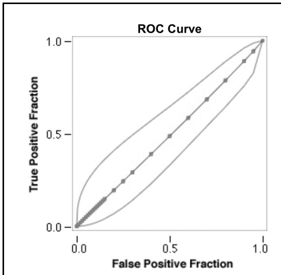
Figure1: ROC curve SIRS \geq 2 score in predicting ICU mortality showing AUC 0.49; 95% CI 0.37-0.61.
