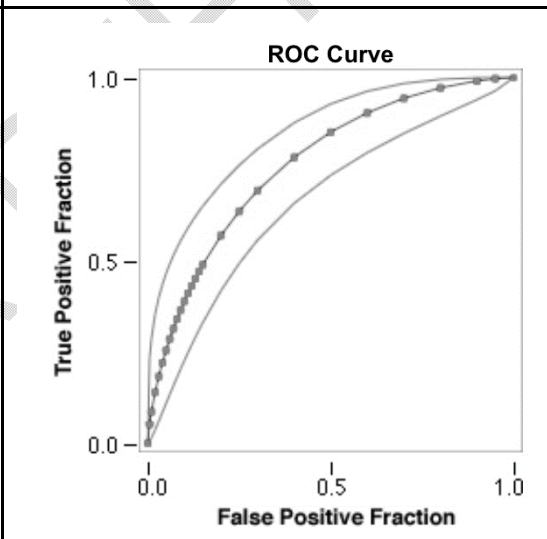
Figure4: ROC curve MEWS \geq 5 score in predicting ICU mortality showing AUC 0.76; 95 % CI 0.68-0.84.
