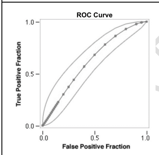
Figure3: ROC curve NEWS \geq 5 score in predicting ICU mortality showing AUC 0.61; 95% CI 0.52-0.71.
