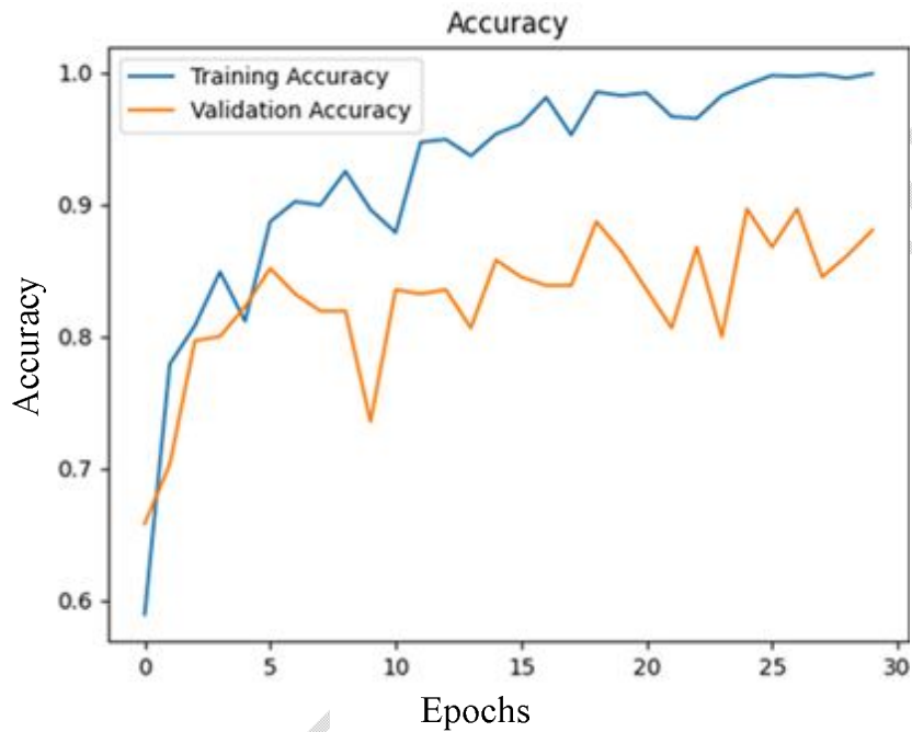
Fig. 8. Graph of accuracy of the proposed method
