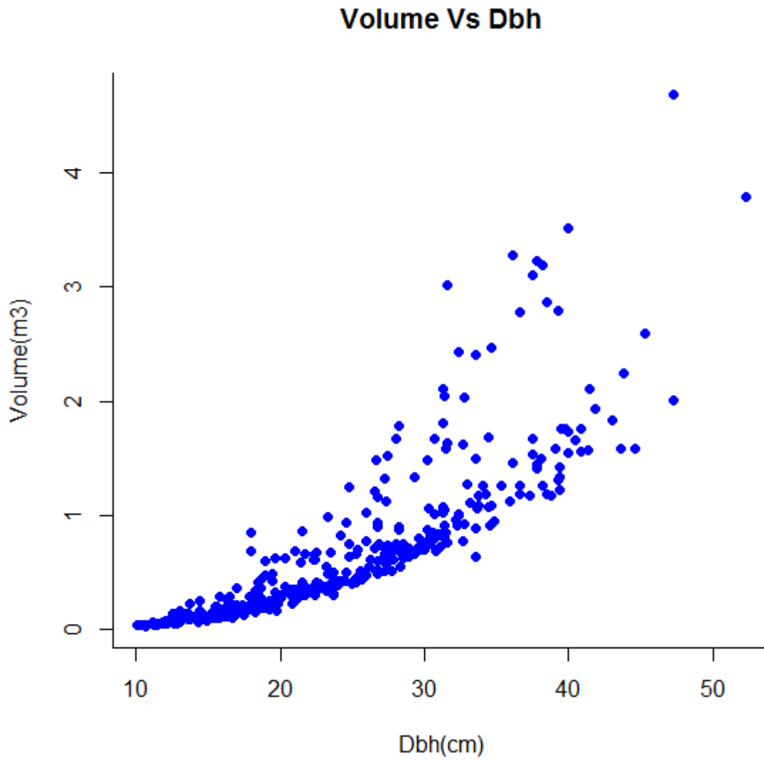
Fig 1: Volume versus diameter at breast height (DBH) for Gmelina trees
