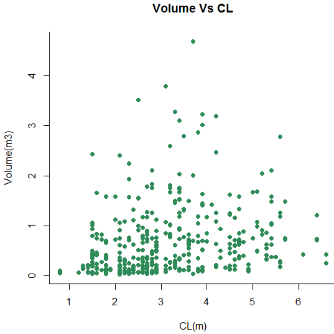
Fig 3: Volume versus crown length for Gmelina trees
