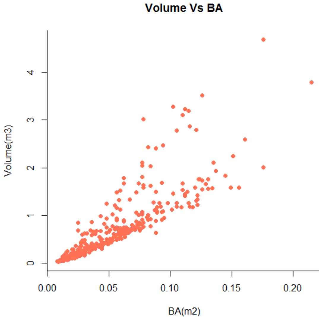
Fig 4: Volume versus basal area for Gmelina trees
