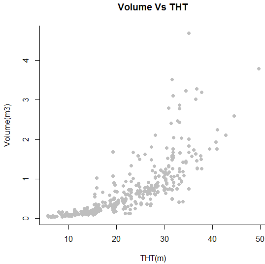
Fig 2: Volume versus total height for Gmelina trees
