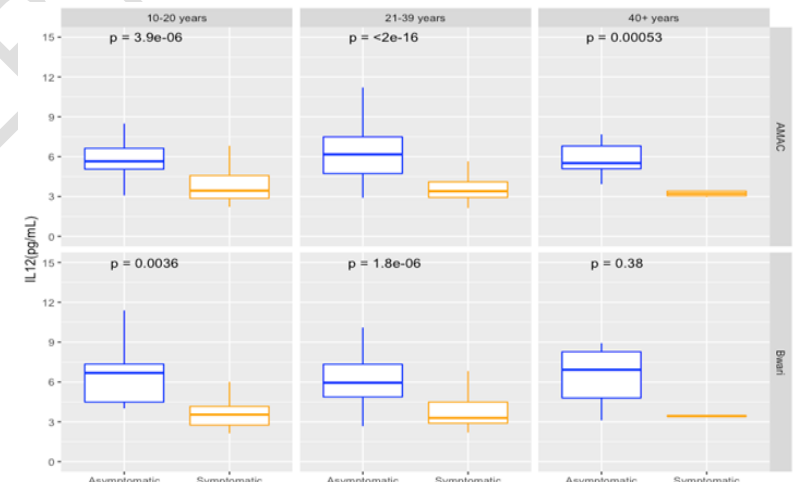
IL-12 (pg/mL)
