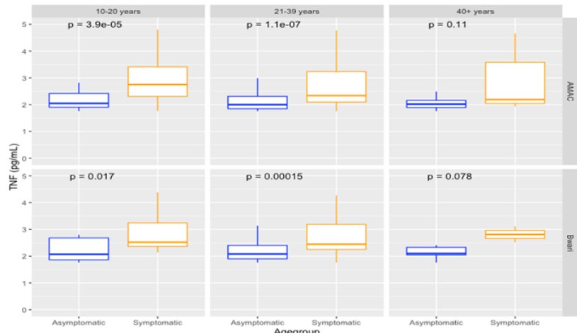
TNF (pg/mL)
