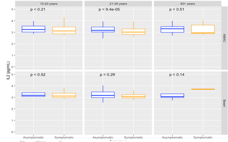
IL-2 (pg/mL)
