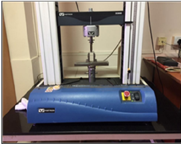
Figure 2 – Load deflection rate test was conducted in Instron® Machine Model no. 3366 used to test each wire with a 3-point method (CIPET) mysuru.
