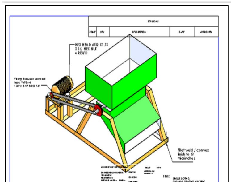
Figure 3: The 3D model drawing
