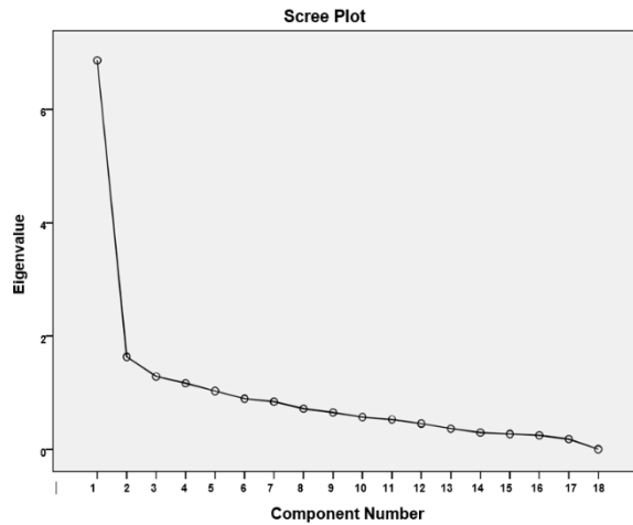
Fig-1: Scree plot
