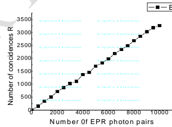
Figure (3): A plot diagram of the number of total coincidences R versus the number of EPR photon pairs.
