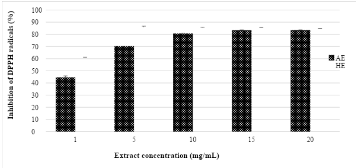
FIGURE 1 Inhibition percentage of DPPH radicals of the aqueous and hydroethanolic extracts from mangosteen fruit peels.
