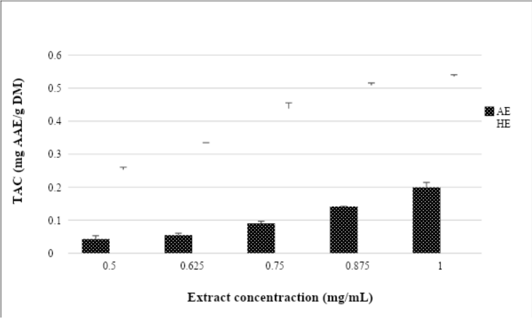
FIGURE 3 Total antioxidant capacity of the aqueous and hydroethanolic extracts of mangosteen fruit peels.
