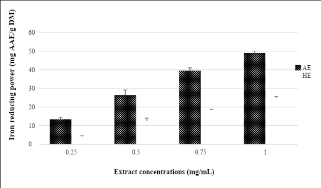
FIGURE 2 Iron reducing power of the aqueous and hydroethanolic extracts of mangosteen fruit peels.
