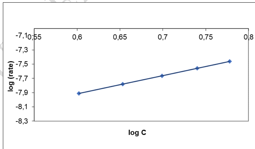
Figure 5. Calibration graph for the initial rate method.
