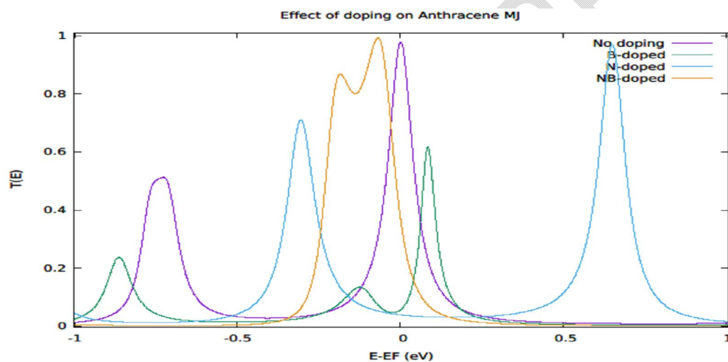
Figure 5: Transmission coefficients of B-doped, N-doped and NB-doped anthracene MJ
