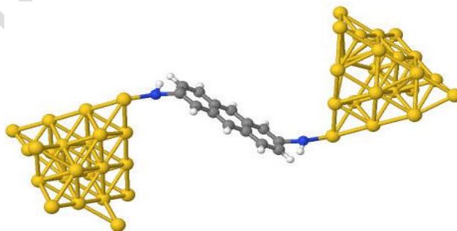
Figure 1: Anthracene molecular junction connected to Au(111) electrodes via Amines anchoring group.
