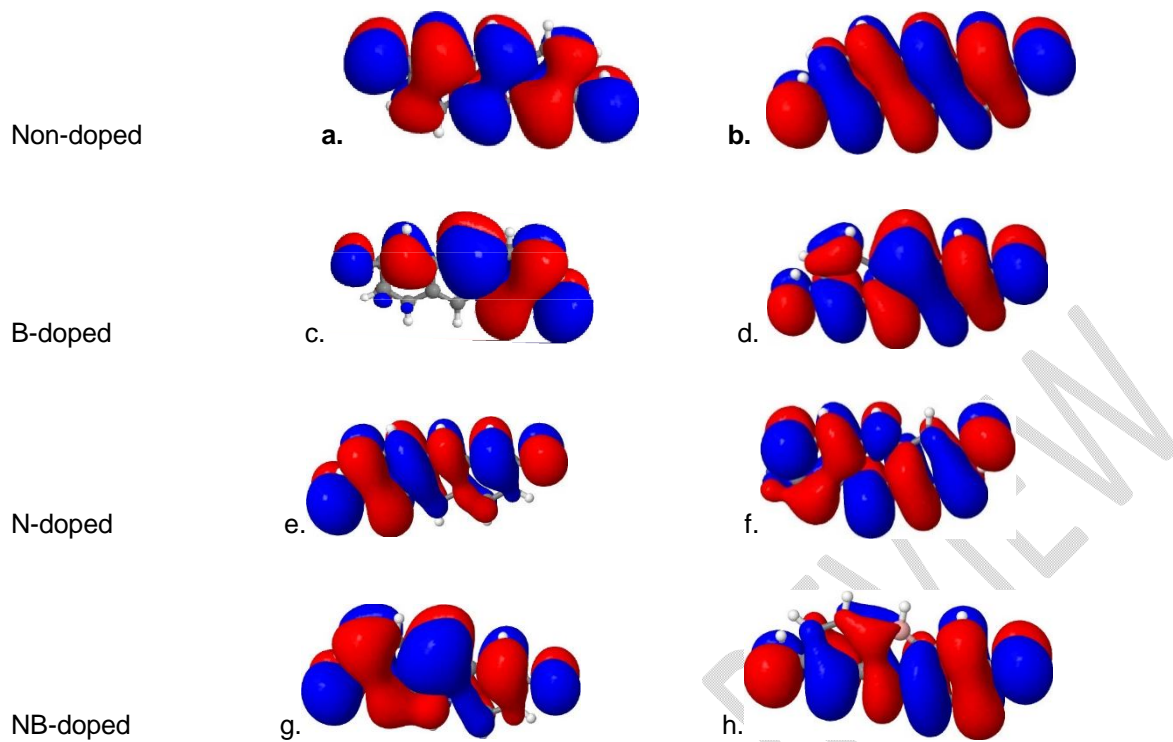
Figure 4: Frontier molecular orbitals for doped and non-doped anthracene
