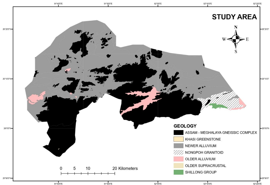
Fig.1. Generalized geological map of the Shillong plateau showing the location of Guwahati, study area (GSI data)
