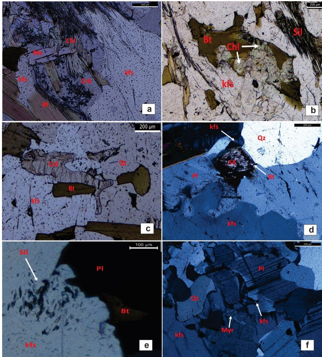
Fig.3 (a) Symplectitic intergrowth of muscovite + chlorite within the decomposed core of finitized cordierite. (b) Pseudomorph replacement of cordierite by K-feldspar + biotite + chlorite. Note that biotite alters into chlorite. (c) Inclusion of altered cordierite grains within the thick rim of K-feldspar + biotite indicates the replacement of cordierite due to the K-activity of the prevailing fluid phase. (d) Formation of the thin rim of K-feldspar at the equilibrium contact of sillimanite and quartz. Note the paucity of matrix sillimanite in another part of the thin section. (e) Presence of tiny inclusions of sillimanite within K-feldspar indicates a paucity of matrix sillimanite. (f) Penetration of k-feldspar along the fracture plane of deformed metamorphic plagioclase grain with albite - twin. Note the presence of inclusions of sub-
