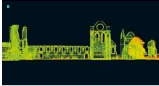
Fig. 13. An orthographic point cloud image displayed with intensity values and silhouette shading Picture by courtesy of Historic Environment Scotland [1]
