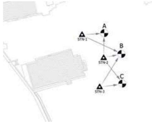
Fig. 11. Illustrative diagram of target arrangement on site
