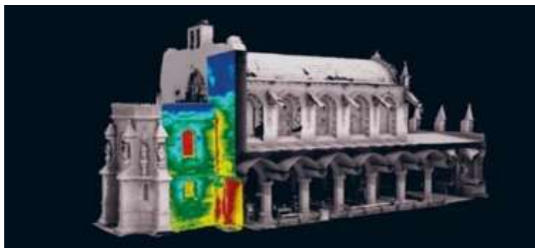
Fig. 25. Thermography overlaid on top of the 3D mesh of Rosslyn Chapel Picture by courtesy of Historic Environment Scotland [1]
