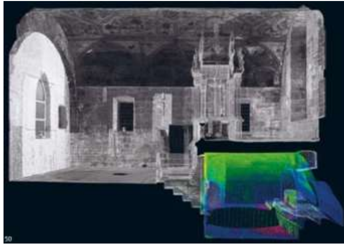
Fig. 24. Cross-section elevation view of Skelmorlie Aisle with crypt showing mapped moisture data Picture by courtesy of Historic Environment Scotland [1]
