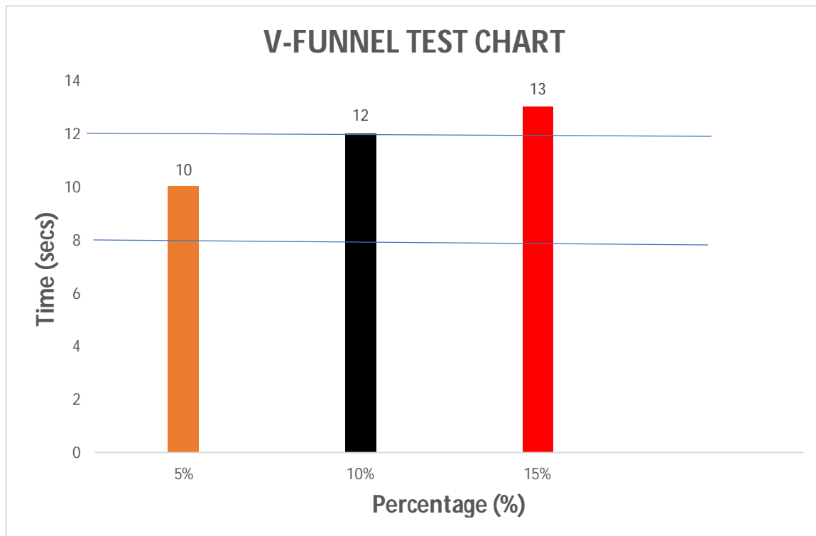
Fig 3: V-Funnel Test Result
