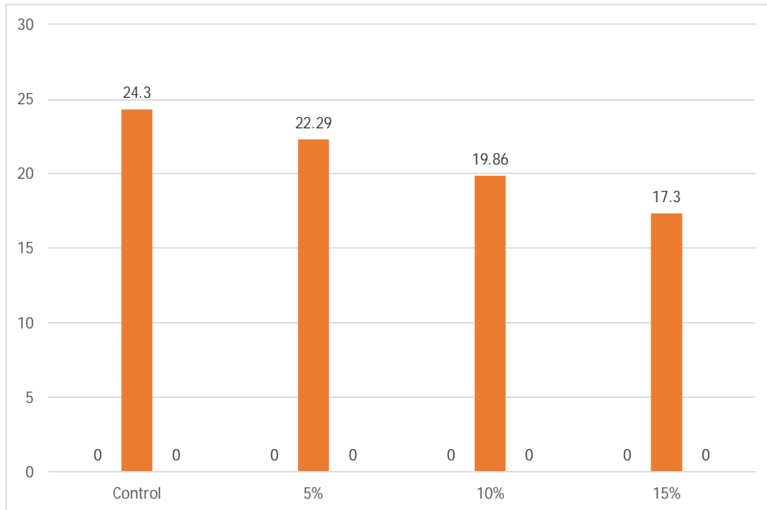
Fig 4: 7-Days Compressive Strength Test Results
