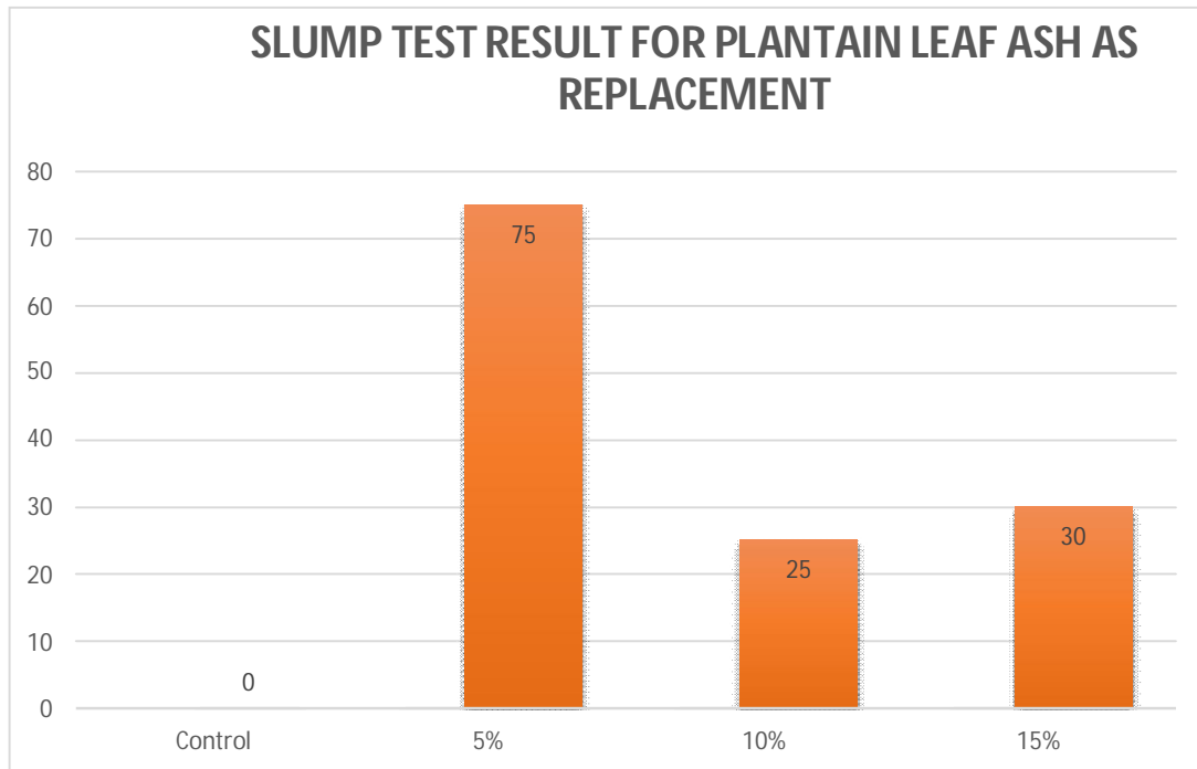
Fig 1: Slump Test Results
