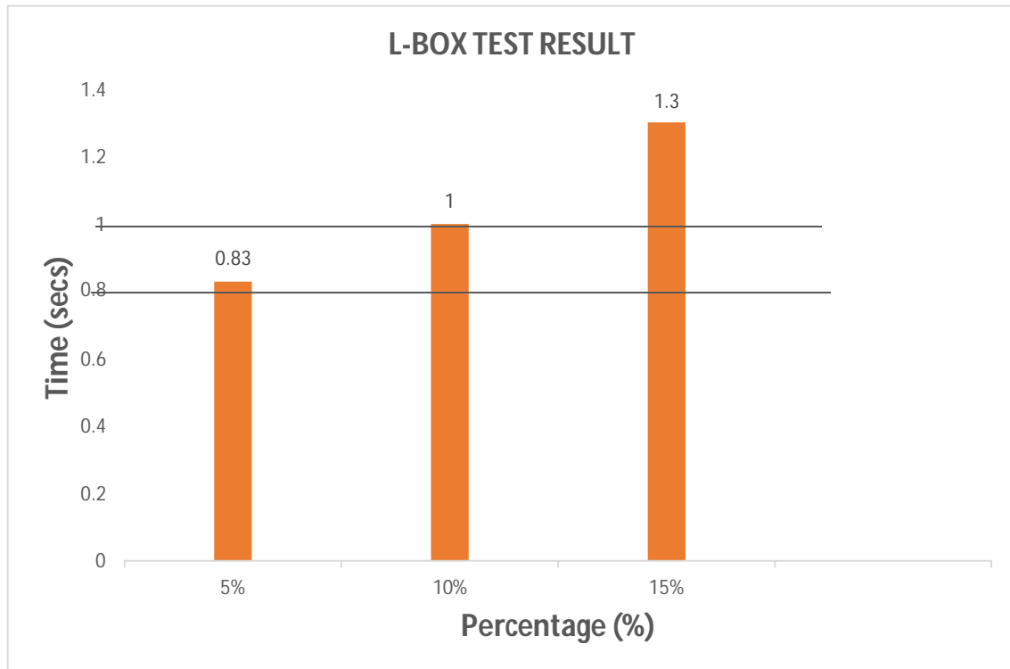
Fig 2: L-Box test result of SCC with PLA
