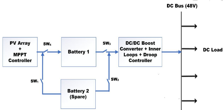
Fig 2. Block Diagram of system chosen
