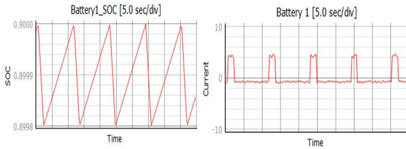
Fig 11. (a) charging discharging of battery 1 (b) flow of current in battery 1
