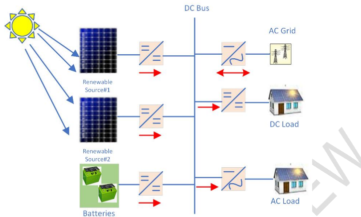
Fig 1. Structure of DC MG
