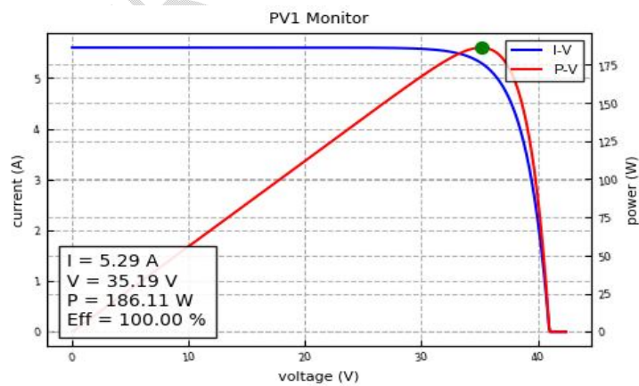
Fig 7: V-I, V-P characteristics at STC
