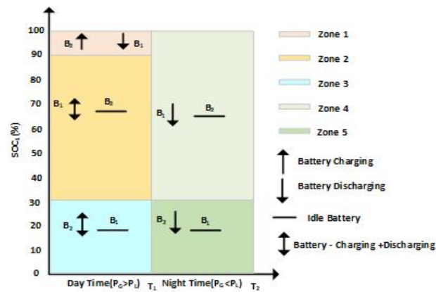
Fig. 6 Zonewise operation of Batteries
