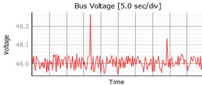
Fig 7. Bus voltage during charging/discharging of batteries
