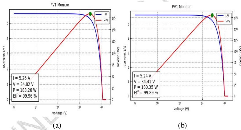
Fig 9: (a) V-I, V-P characteristics for a temperature of 30°C at 1000 watt/m 2 of irradiation (b) V-I, V-P characteristics for a temperature of 30°C at 1000 watt/m 2 of irradiation
