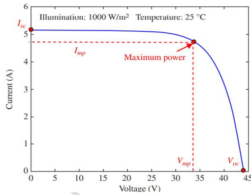
Fig 3. I(V) characteristic of a PV panel
