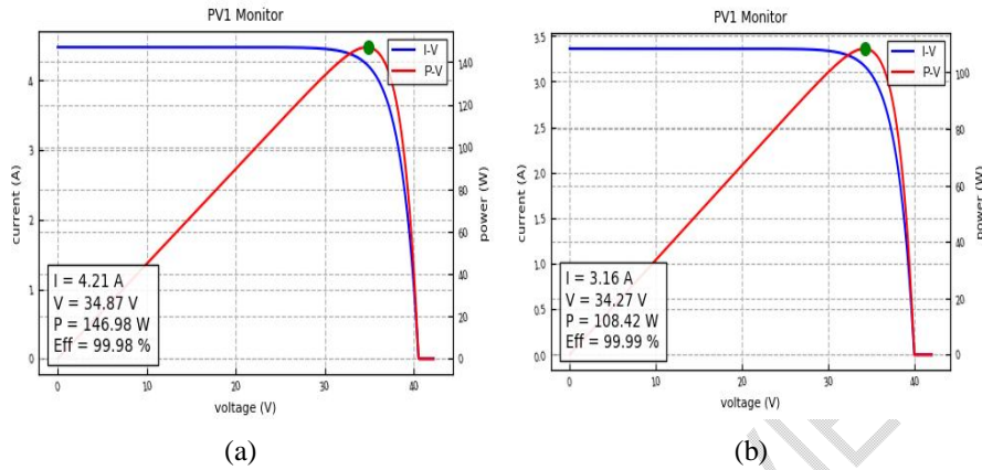
Fig 8: (a) V-I, V-P characteristics for irradiation of 800 W/m 2 at 25°C (b) V-I, V-P characteristics for irradiation of 600 W/m 2 at 25°C.
