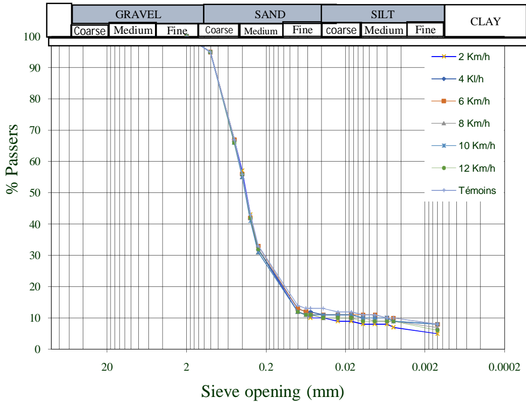
Figure 3: Particle size analysis curve for the different plowing speeds
