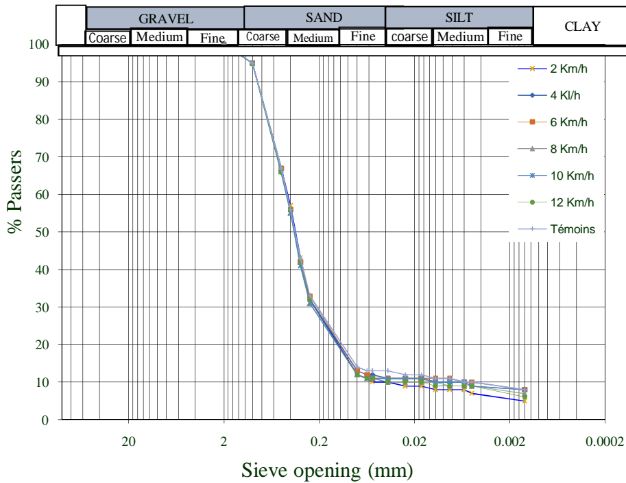
Figure 3: Particle size analysis curve of the different different plowing speeds
