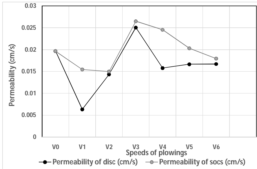
Figure 5: Permeability of plowed-plowed soil to coulters and discs as a function of plowing- plowings speed
