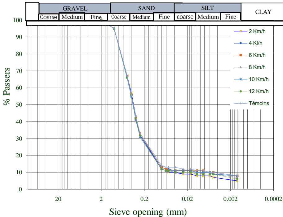
Figure 3: Particle size analysis curve of for the different plowing plowings speeds
