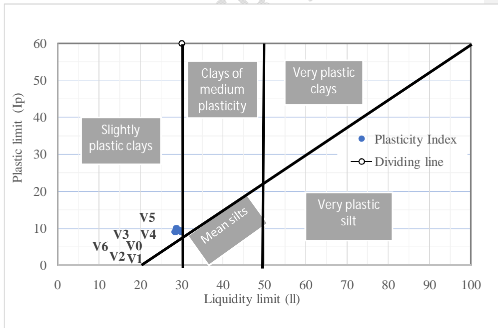
Figure 4: Liquidity and plasticity limits in the Casagrande plasticity diagram
